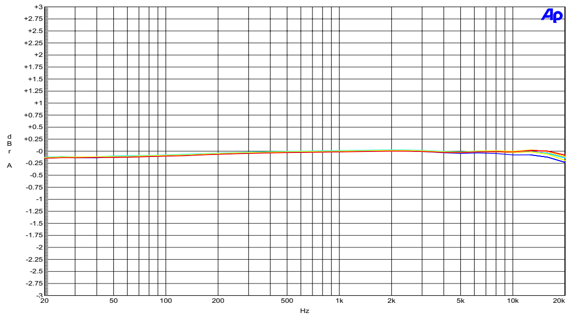
FIGURE 3: Frequency Response
