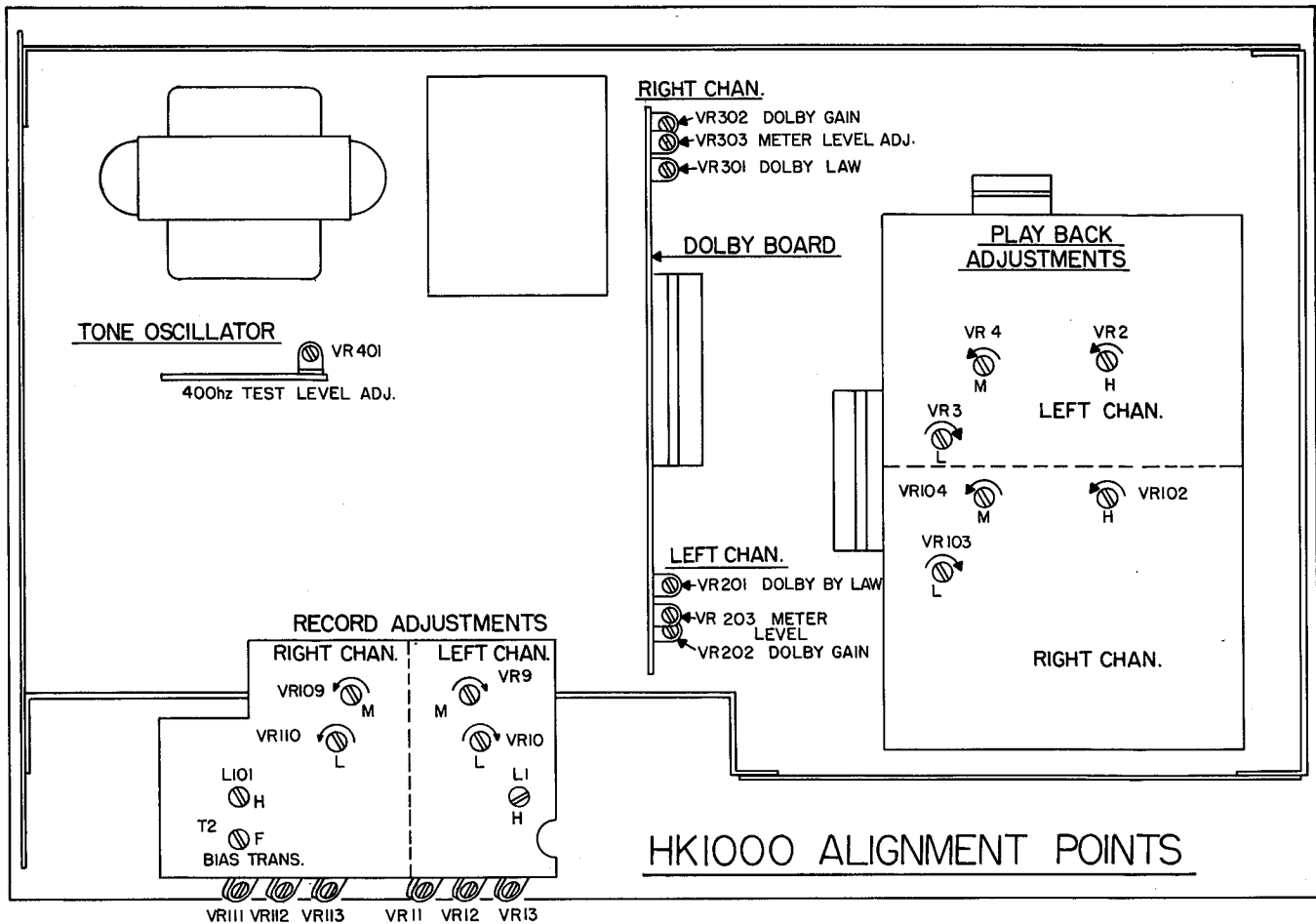
BOTTOM VIEW
