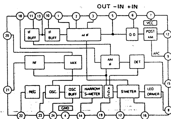
Block Diagram
