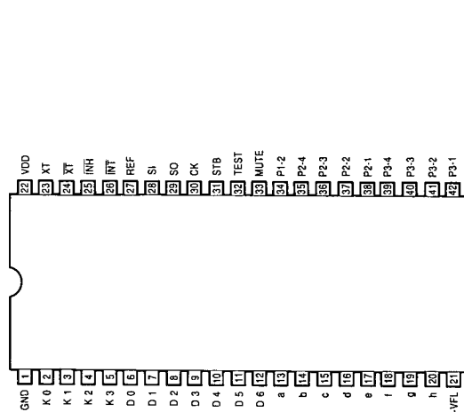
IC701 : T9301AN-020 FL DRIVER and PLL CONTROL
