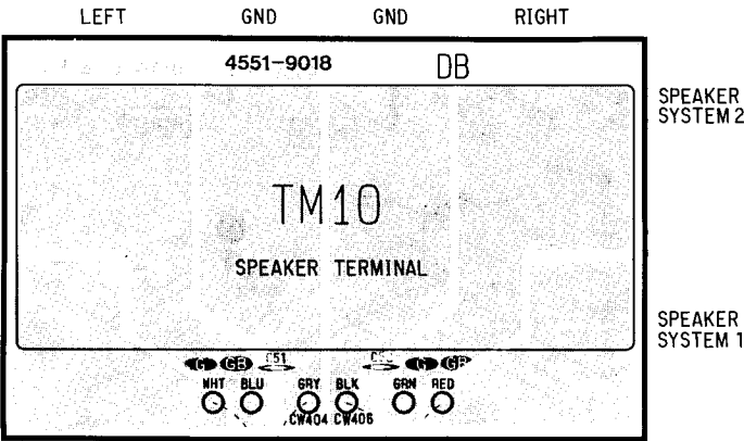
PCB-2 Speaker P. C. Board
