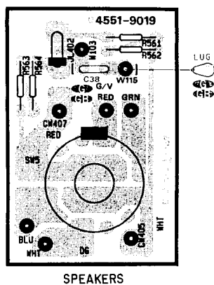
PCB-5 Speaker Switch P. C. Board
