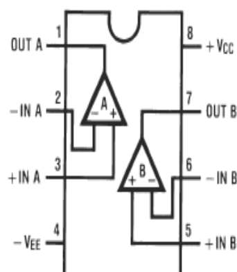
LM833M, pre-amp, SMD
