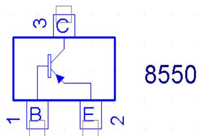
8550, PNP Transistor, SMD
