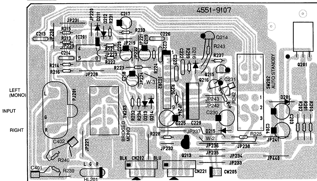
PCB-2 Auto On/Off P.C.Board
