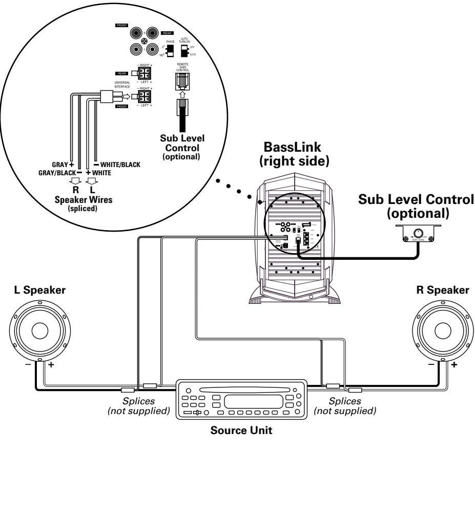
Figure 10. BassLink audio connections for a head unit equipped with two speaker-level outputs.
