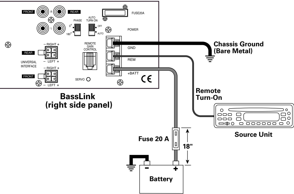
Figure 5. Power connections for BassLink.
