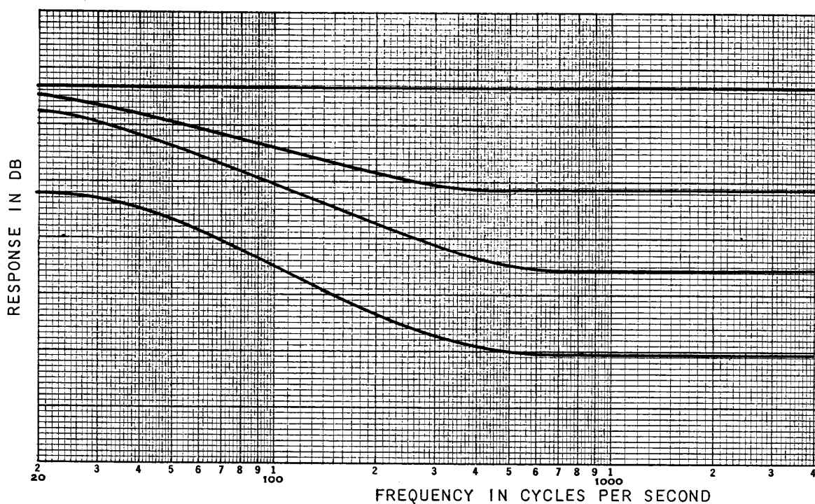
FIGURE 3-4 LOUDNESS COMPENSATION
