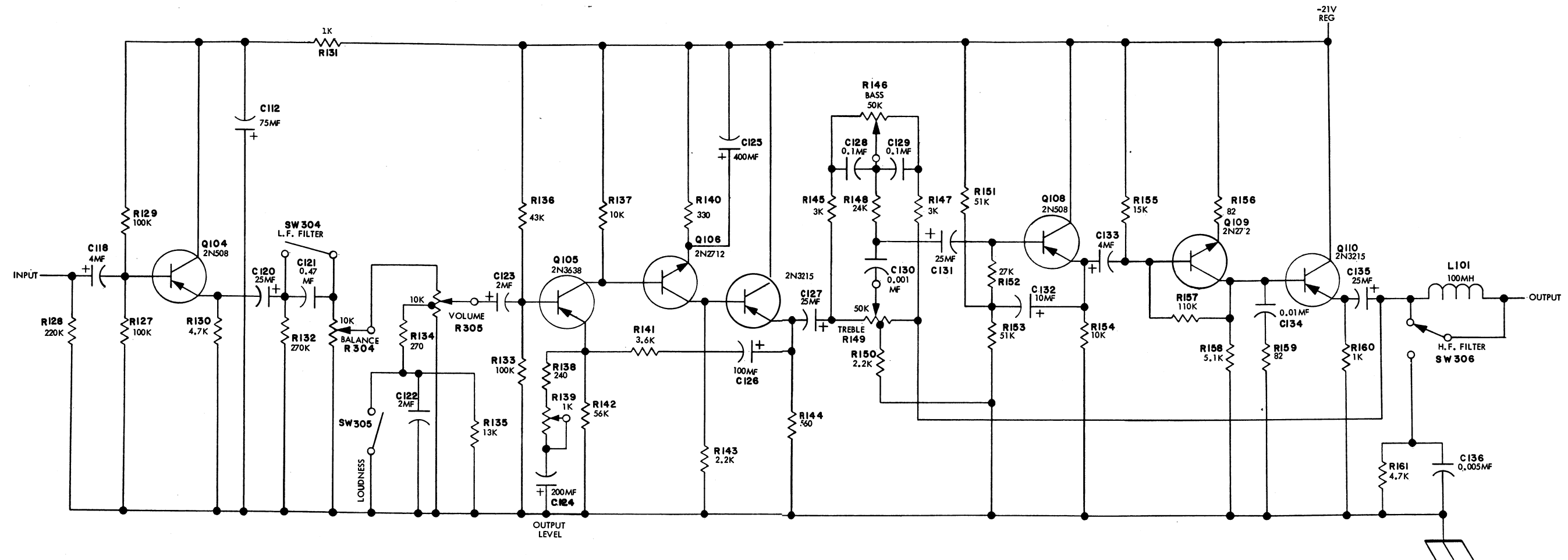
LINE AMPLIFIER
