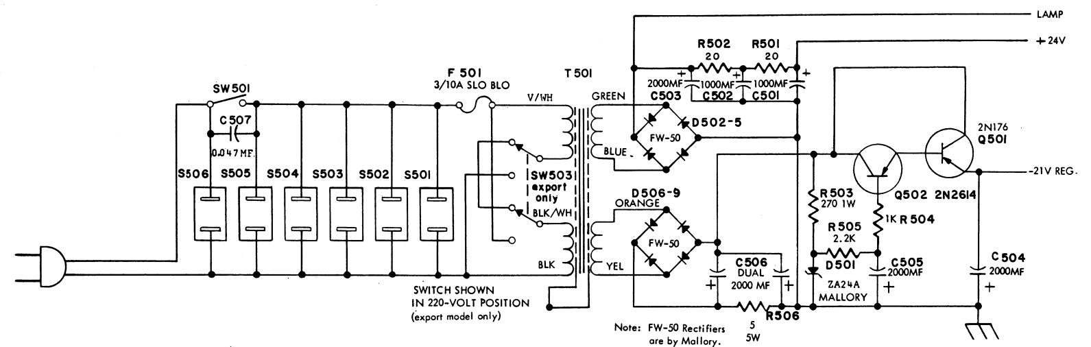
POWER SUPPLY ASSEMBLY
