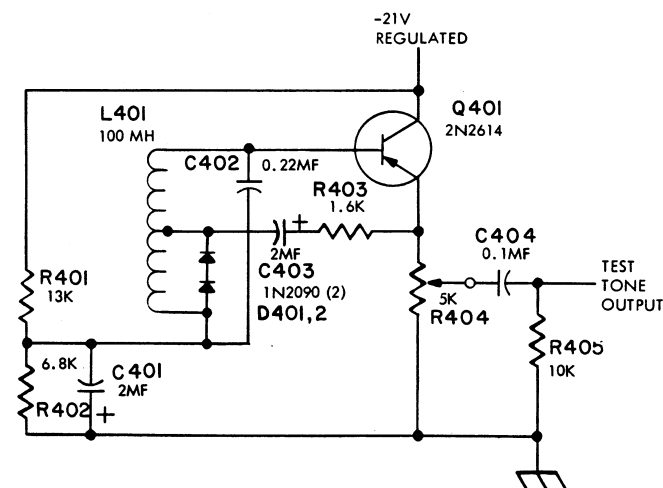
TONE OSCILLATOR
