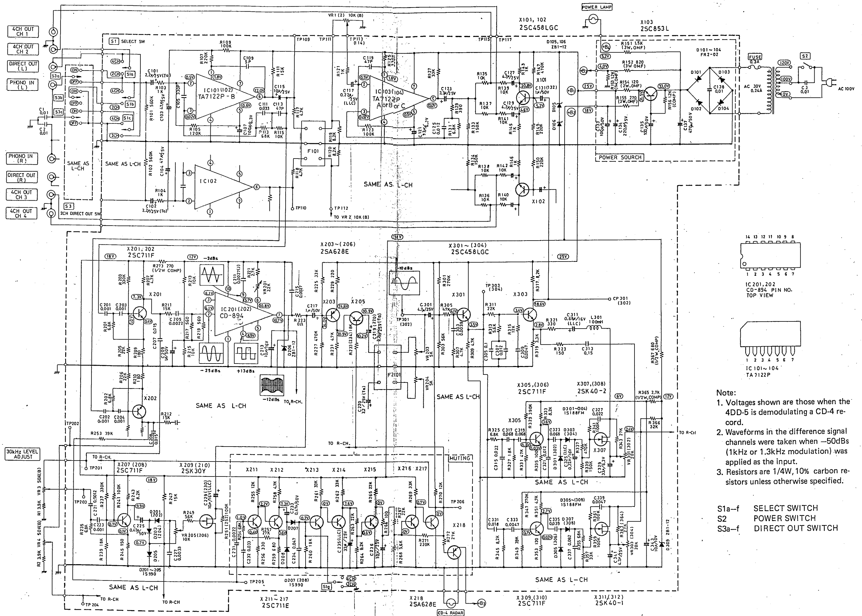
4DD-5 Circuit Diagram
