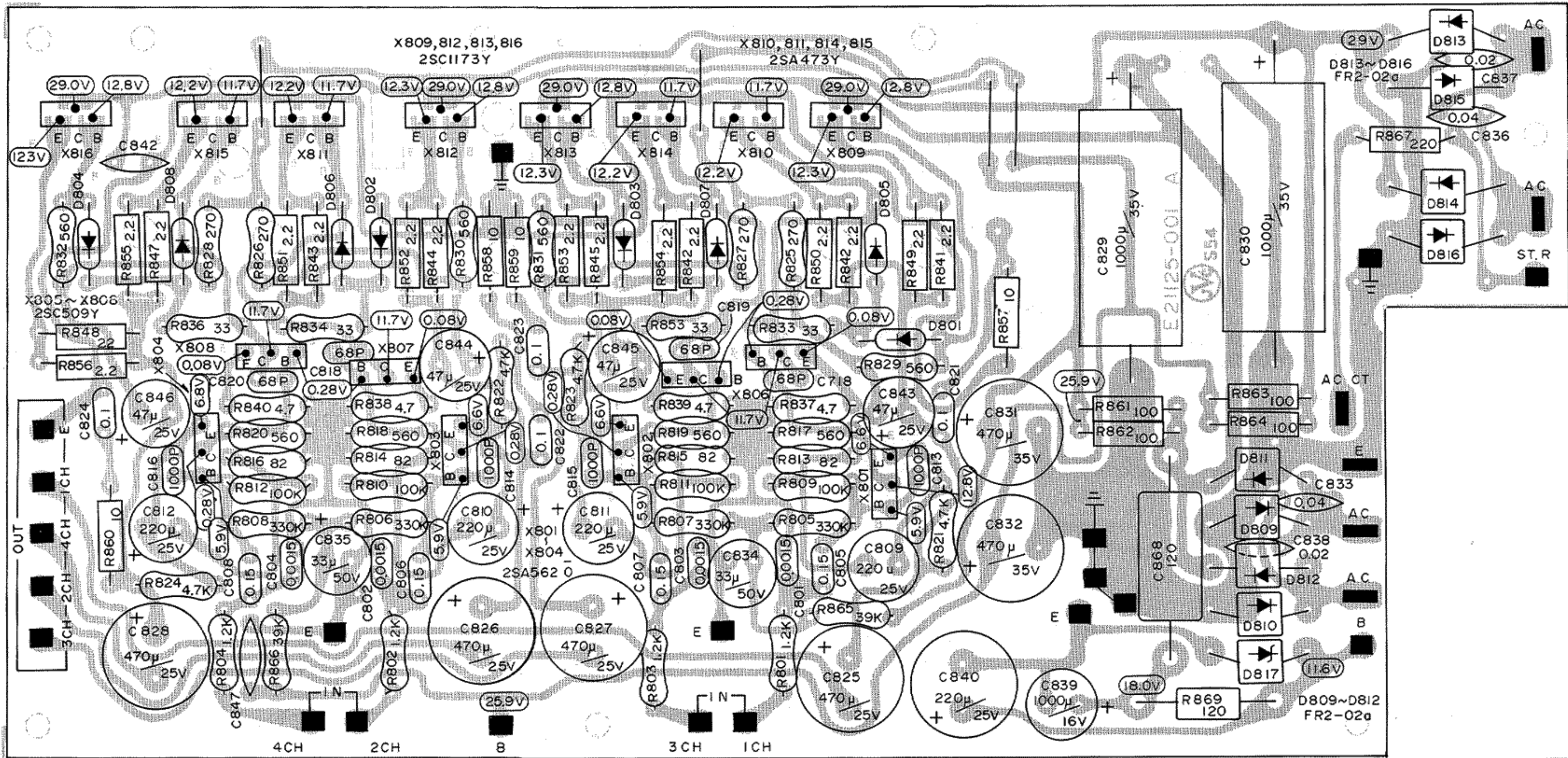
Fig. 19 Bottom View
