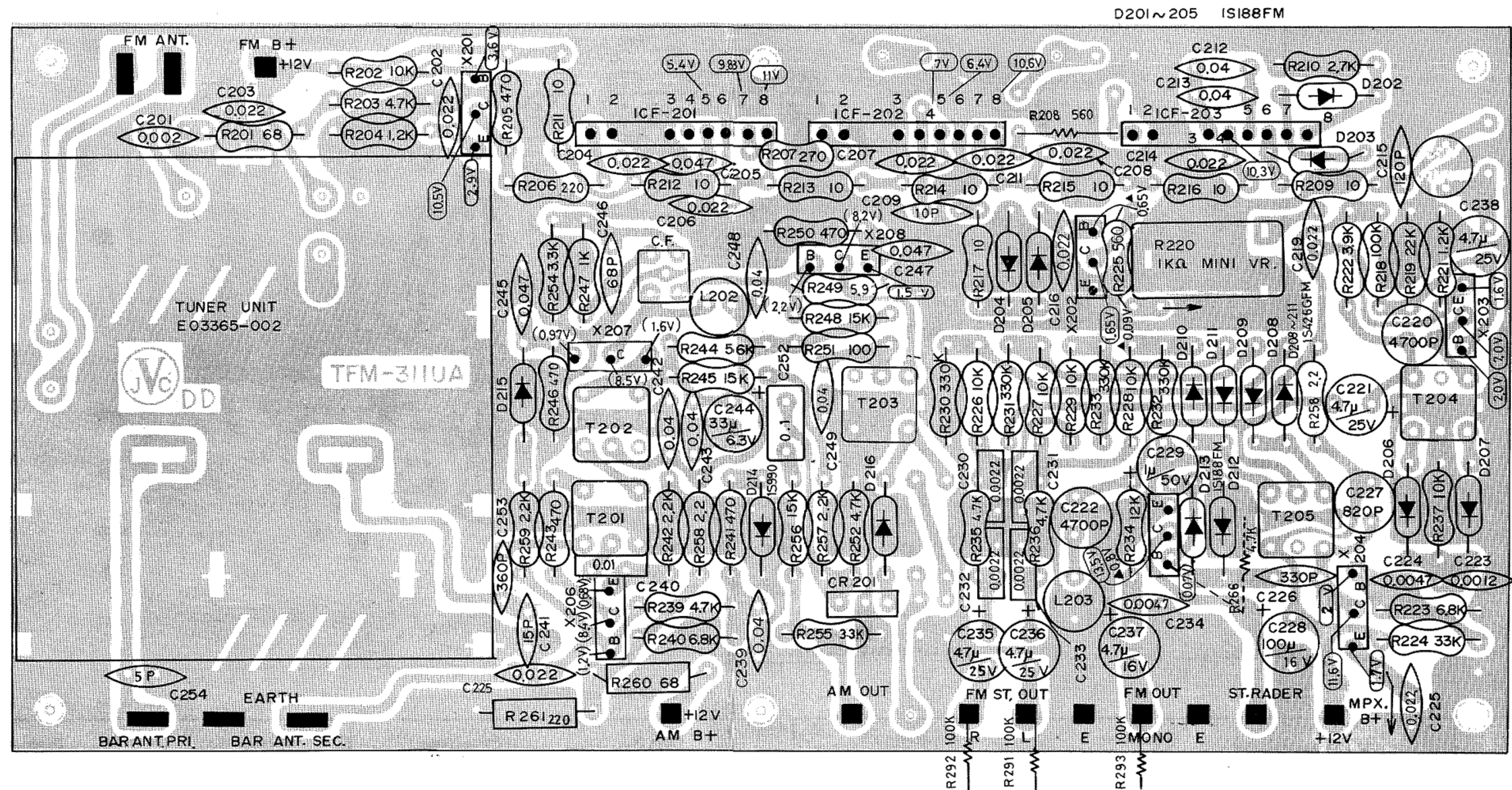
Fig. 20 Bottom View
