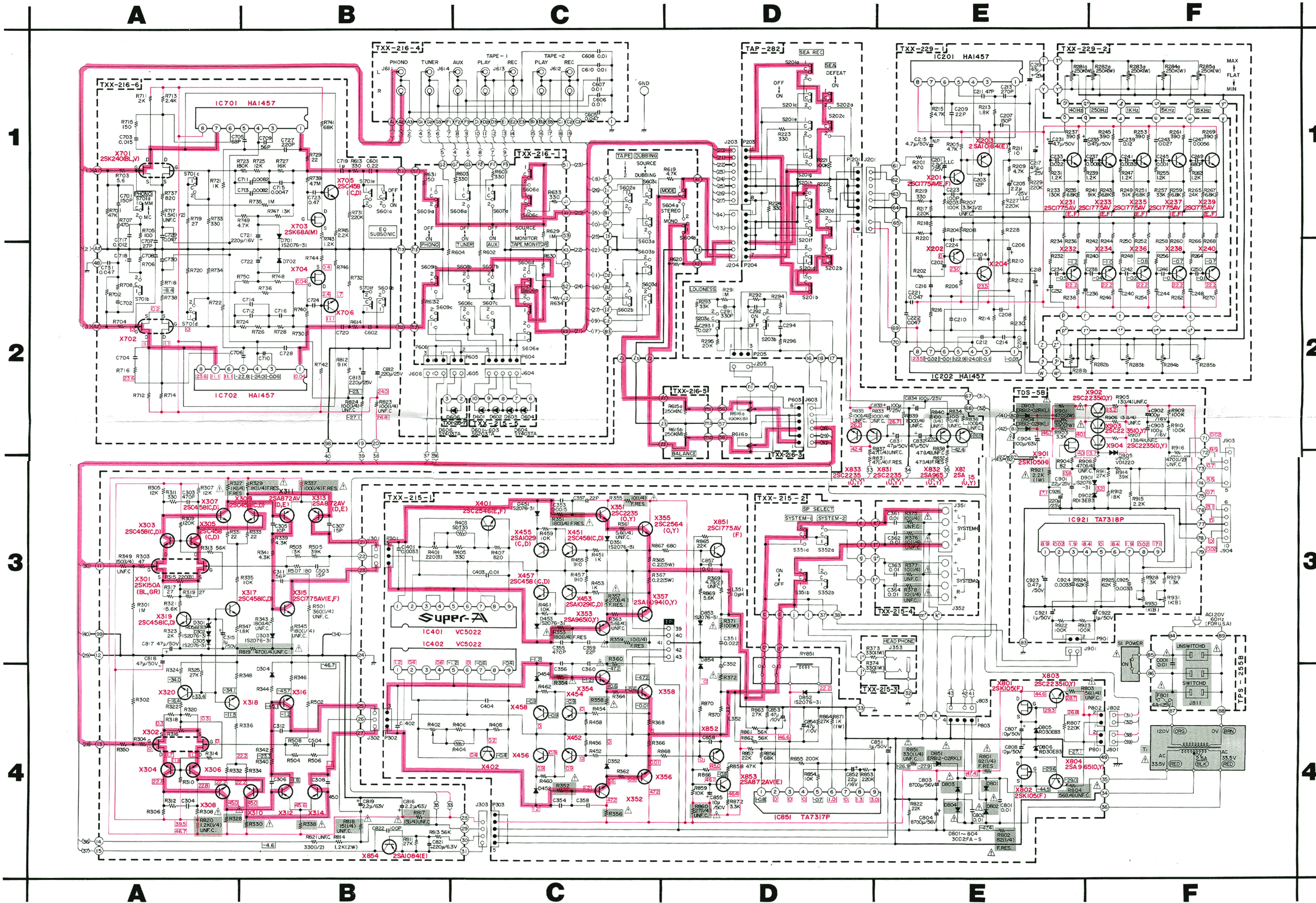
Printed Circuit Board Ass'y Location
