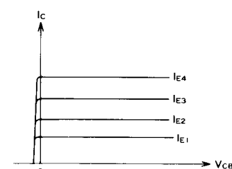
Output characteristics of common-base amplifier Fig. 10
