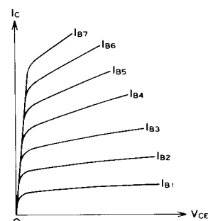
Output characteristics of common-emitter amplifier Fig. 8
