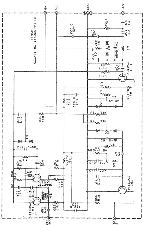
* MARK EF, EN, O BS R149 10K 22K R163, R164 4, 7K 3, 3K R165, R166 NONE USED
