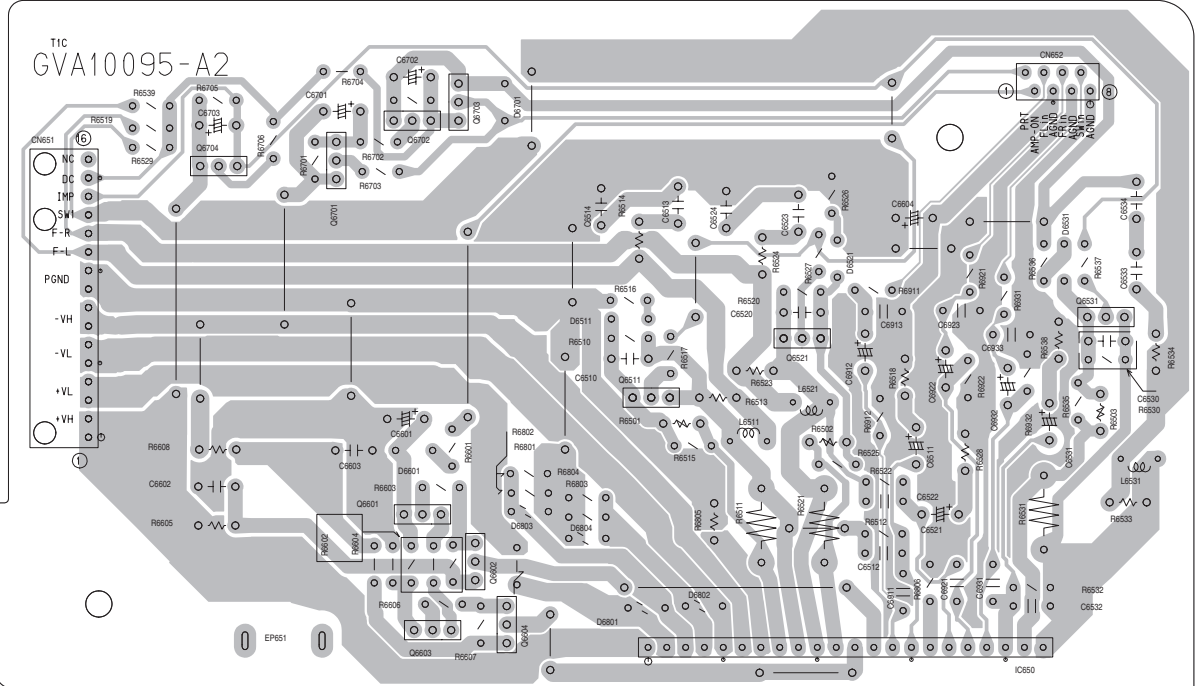
(FL board)
