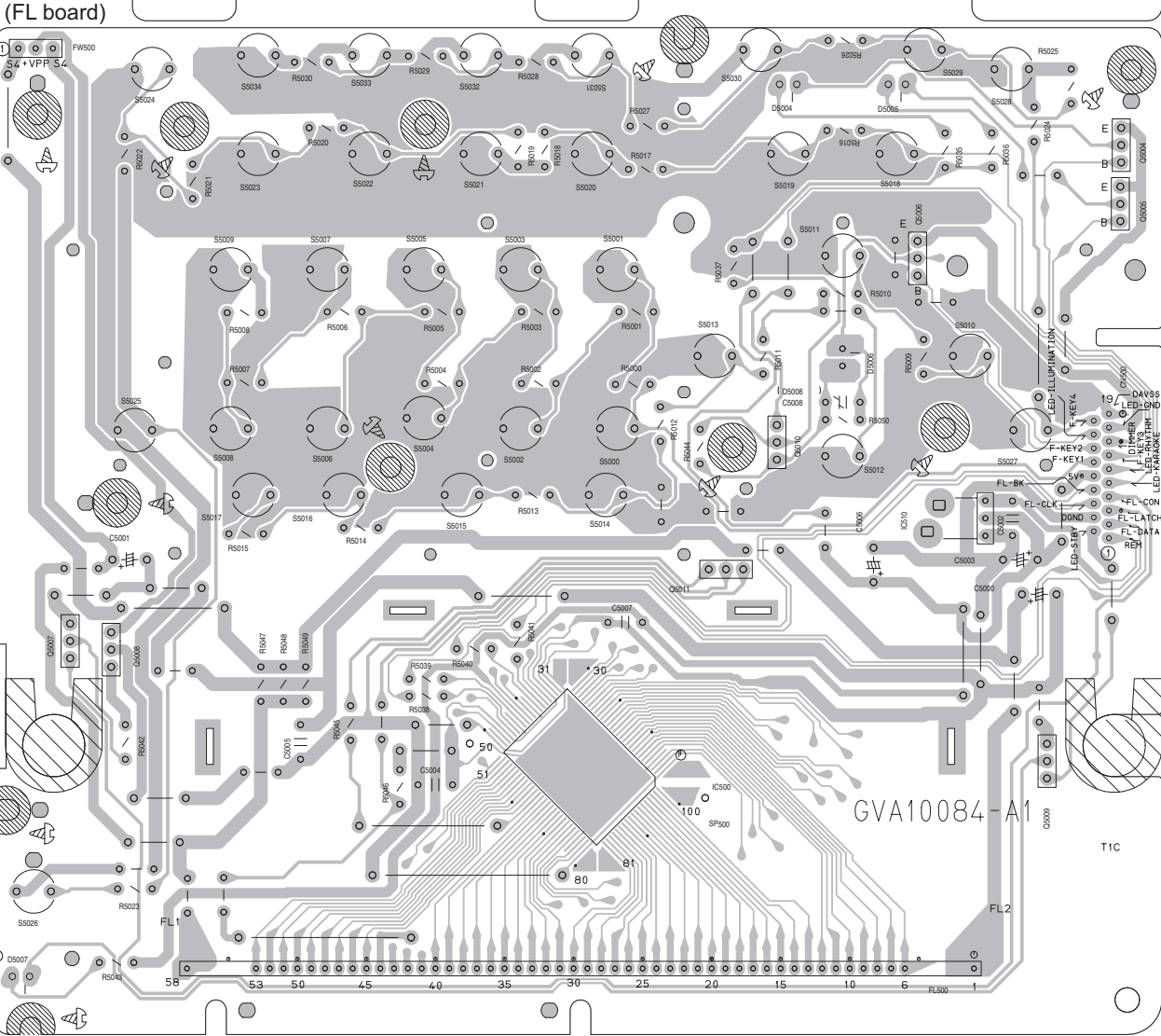
(FL board)
