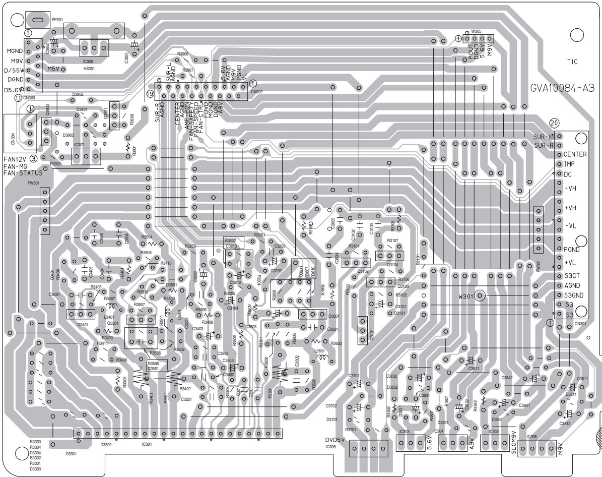
(Amplifier board 1)
