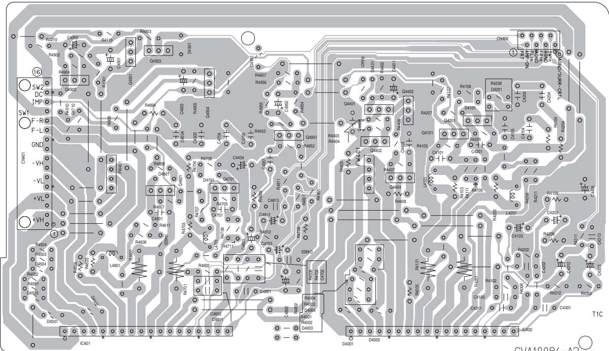
(FL board)
