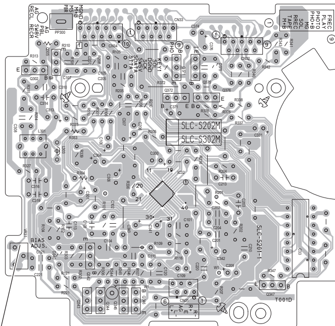
BIAS adjust VR31 (Only B cassette mechanism)
