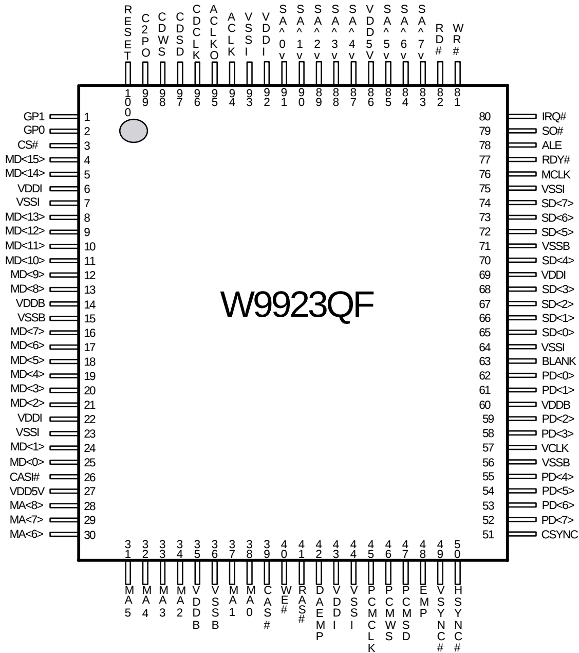
2 Pin function (1/2)
