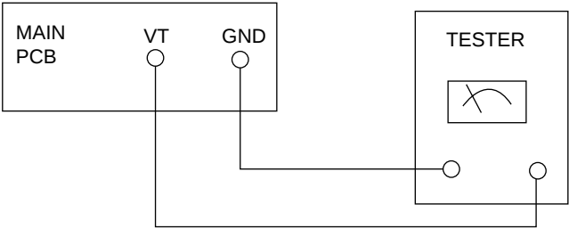
Fig 1-4 OSC Voltage
