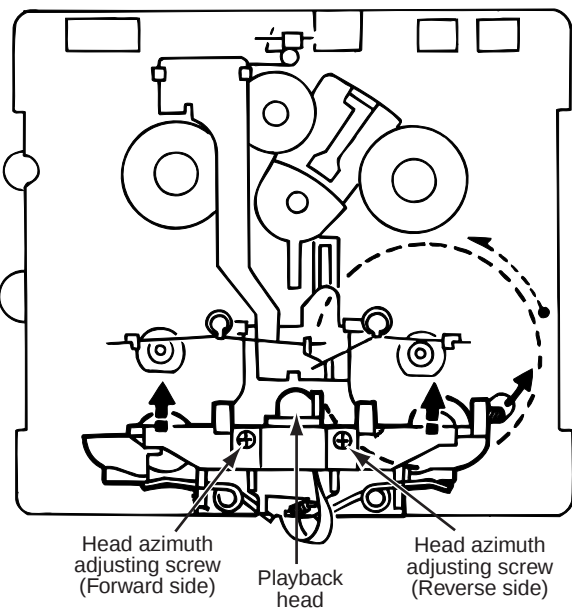
Cassette mechanism section (Mechanism A section)
