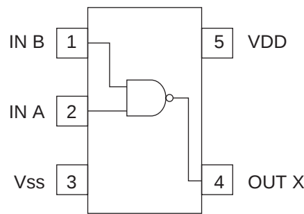
1. Pin layout
