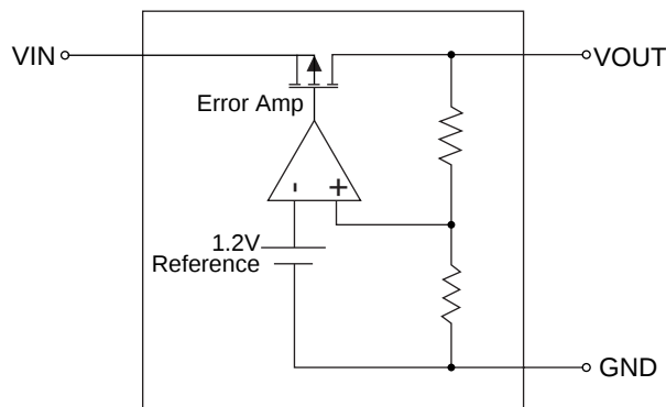
2. Block diagram
