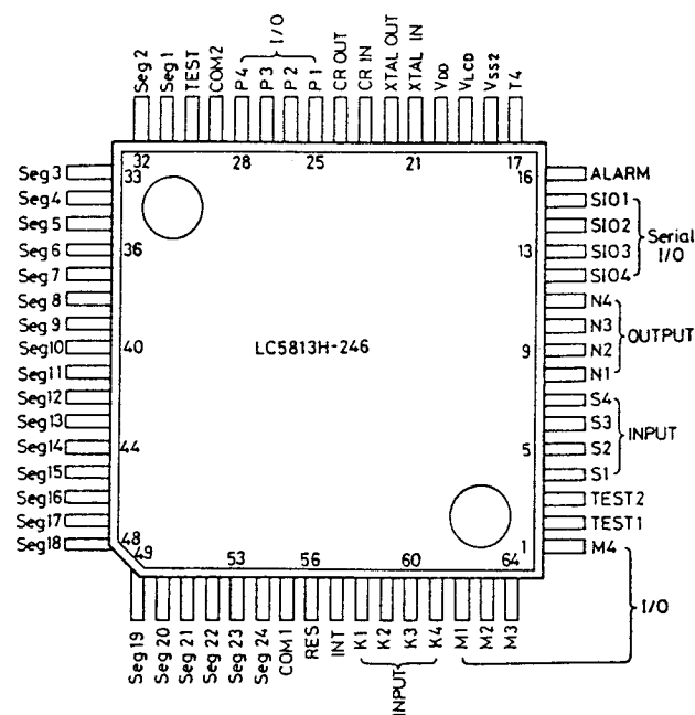
IC421: LC5813H-246
