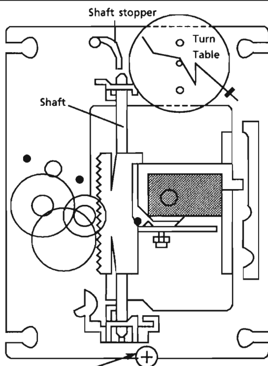
Fig 10 CD mechanism assembly
