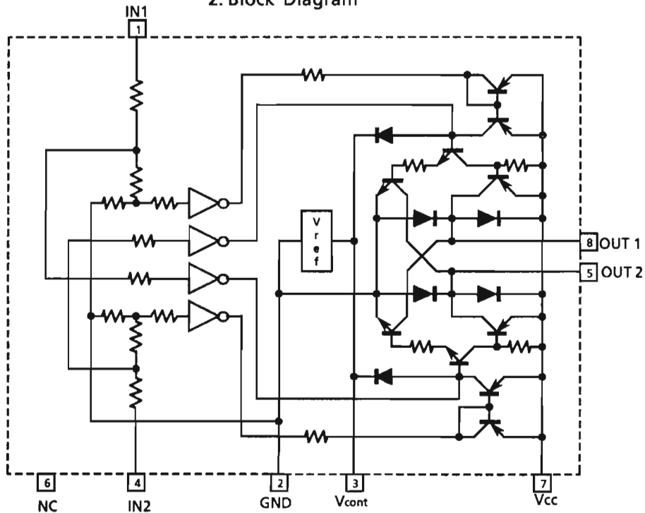
2. Block Diagram
