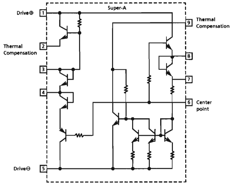
2. Block Diagram
