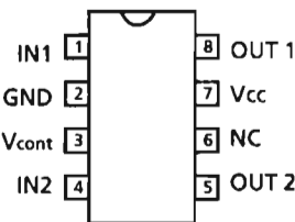
1. Terminal Layout
