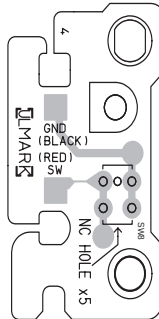
(Switch board)
