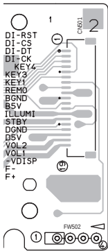
(Front board)
