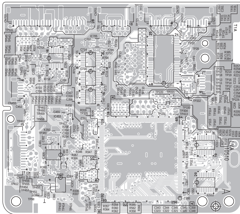
Reverse side
