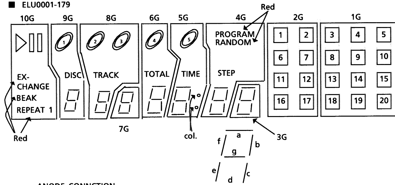
ANODE CONNECTION
