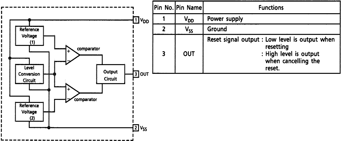
Block Diagram
