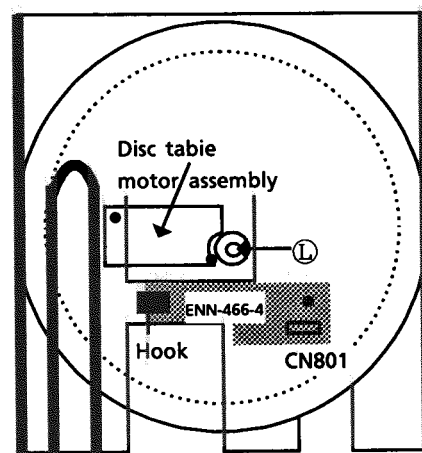
Fig 6 Disc tray bottom view
