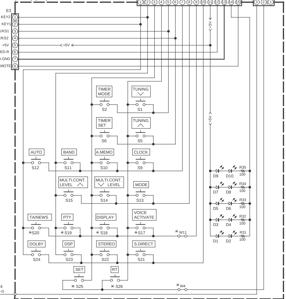
CV-500/V550/V700/V750/V770(K) (6/6)
