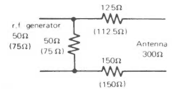
Fig. 2 Dummy Antenna
