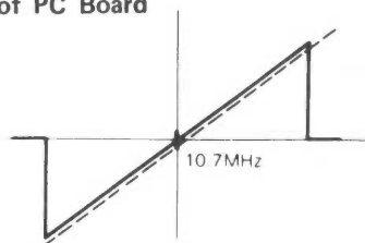
Fig. 5 DISCRI Wave Form
