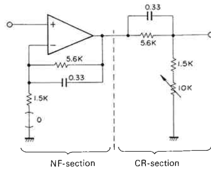
Fig. 10-1 Equivalent circuit for boosted BASS control
