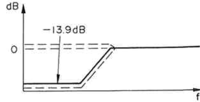
Fig. 9-3 Overall frequency response of decreased BASS control
