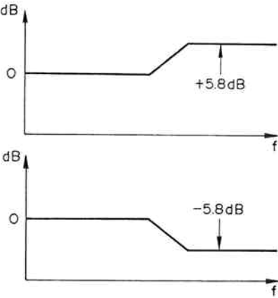
4-2 Frequency response of NF-section (above) and RC-section (below)
