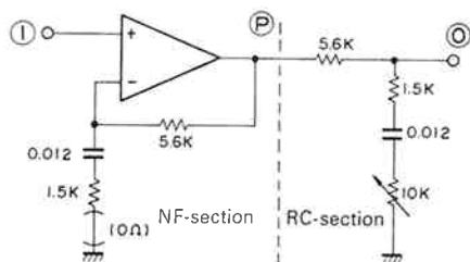
Fig. 6-1 Equivalent circuit for boosted TREBLE control
