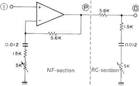
Fig. 4-1 Equivalent circuit for flat TREBLE
