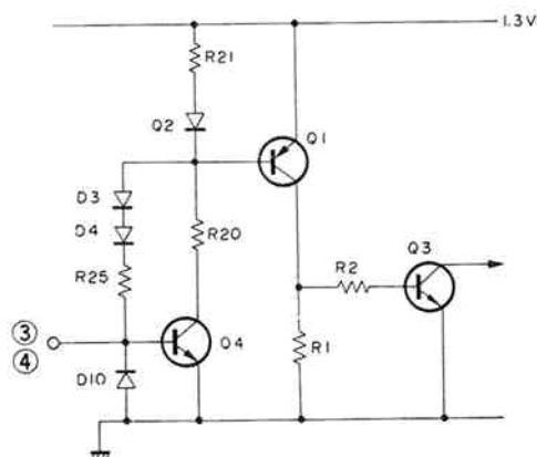
Fig. 11 Zero-potential detector
