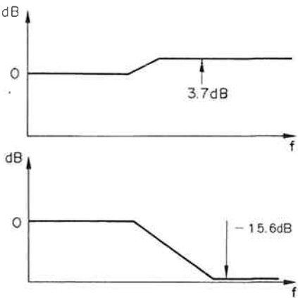
Fig. 5-2 Frequency responses of NF-section (above) and RC-section (below)
