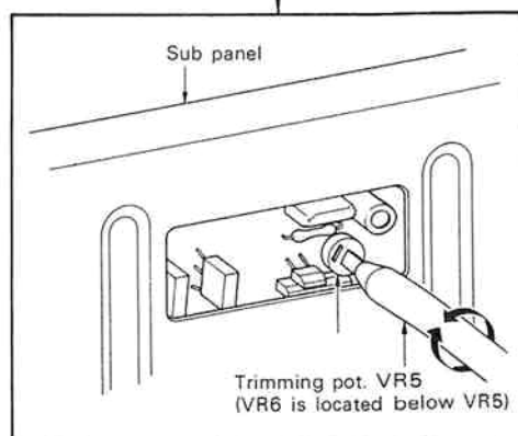
Fig. 2. Power amp offset voltage adjustment.
