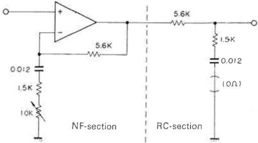
Fig. 5-1 Equivalent circuit for lower TREBLE control setting
