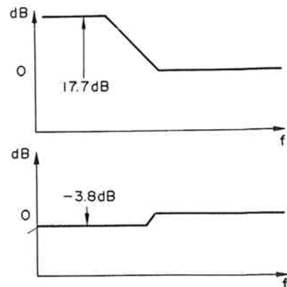
Fig. 10-2 Frequency responses of NF-section (above) and RC-section (below)
