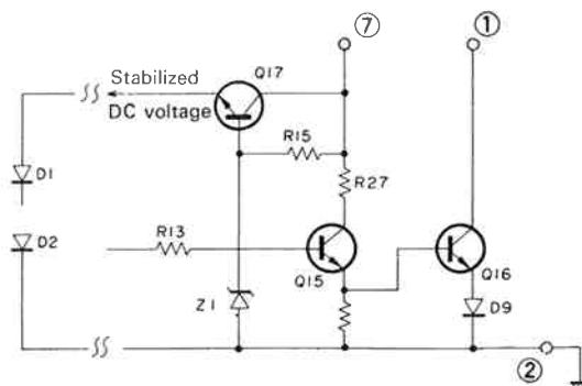
Fig. 15 Relay driver and power stabilizer
