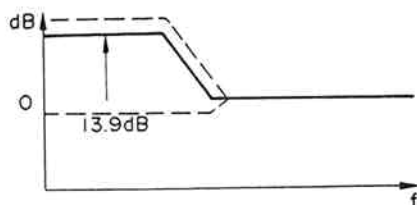
Fig. 10-3 Overall frequency response with boosted BASS control
