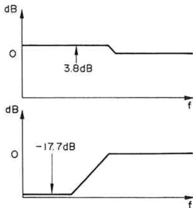
Fig. 9-2 Frequency responses of NF-section (above) and RC-section (below)
