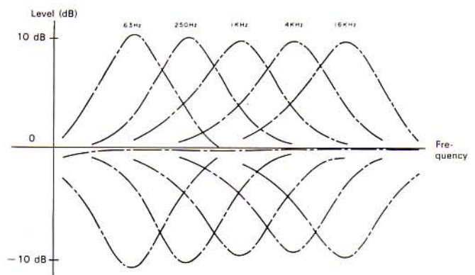
Fig. 3 MAC characteristics
