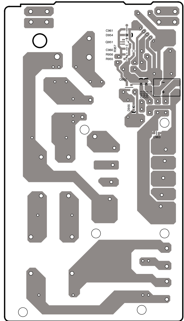
Soldering side view from component side
