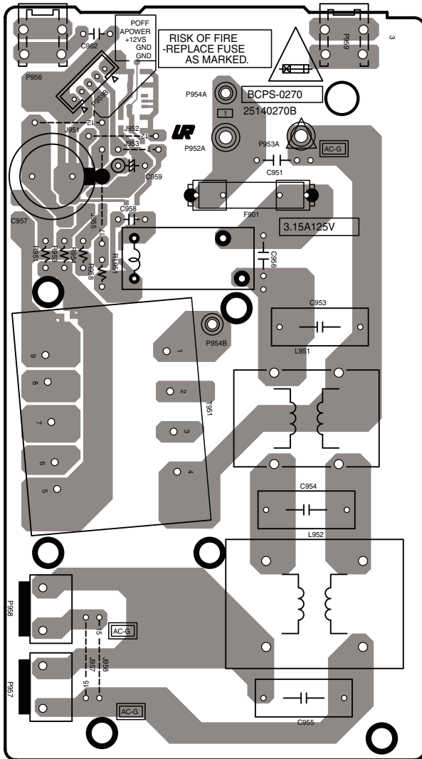
Component side view from soldering side
