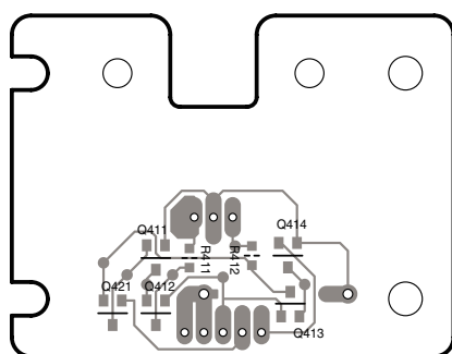
Component side view from soldering side
