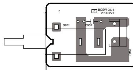
Component side view from soldering side
