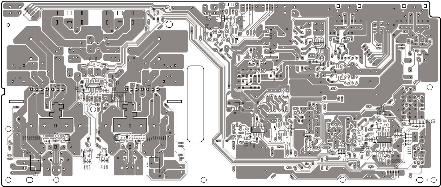
Soldering side view from component side
