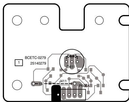
Soldering side view from component side
