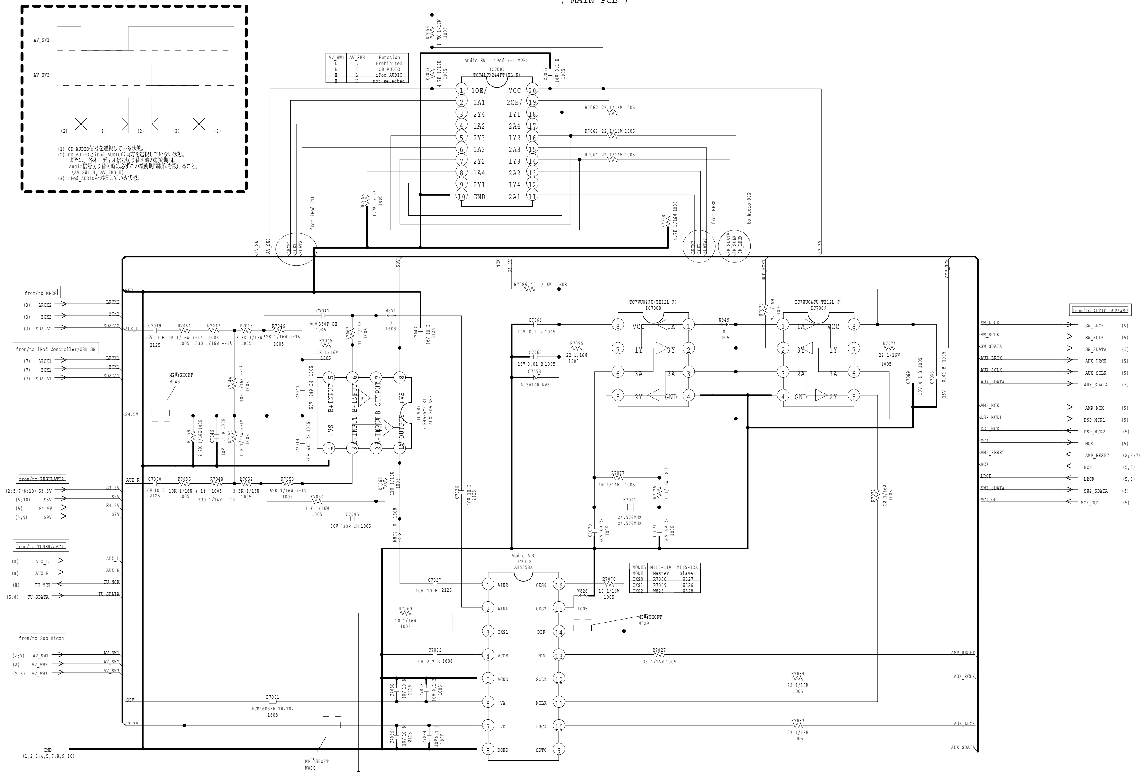
AUDIO SW SCHEMATIC DIAGRAM ( MAIN PCB )
