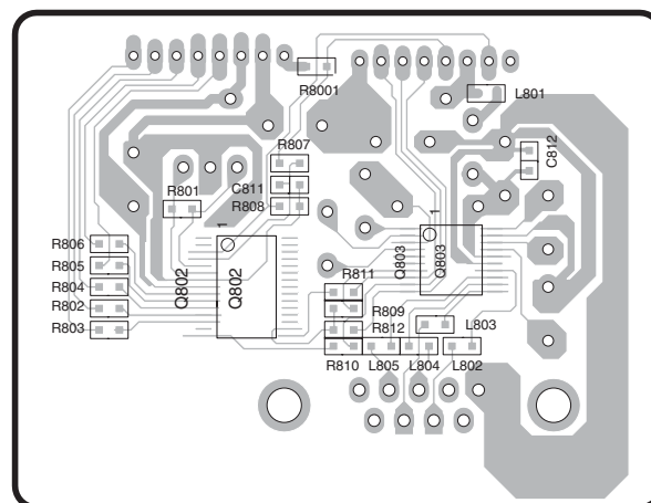
Soldering side
