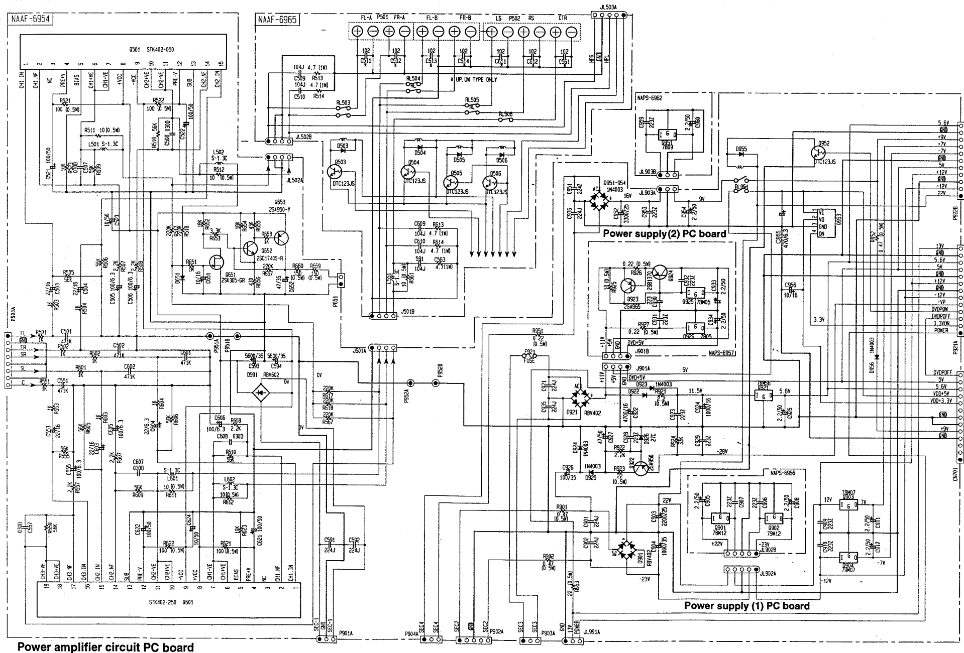
SCHEMATIC DIAGRAM 2
