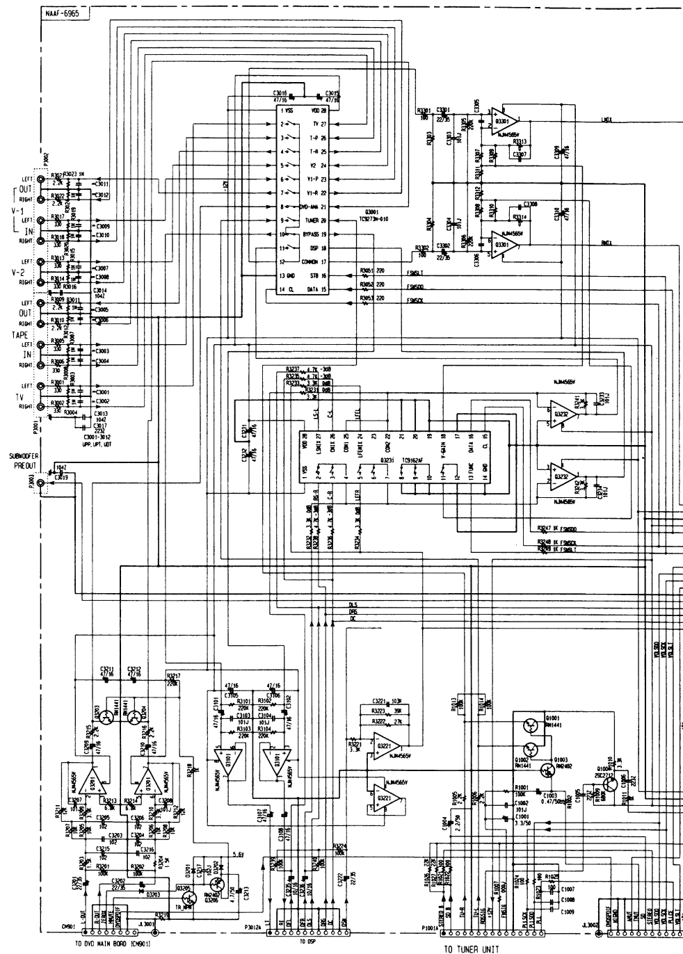
Speaker terminal PC board
