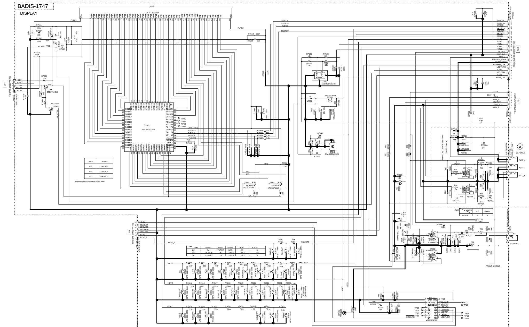
DISPLAY SECTION
