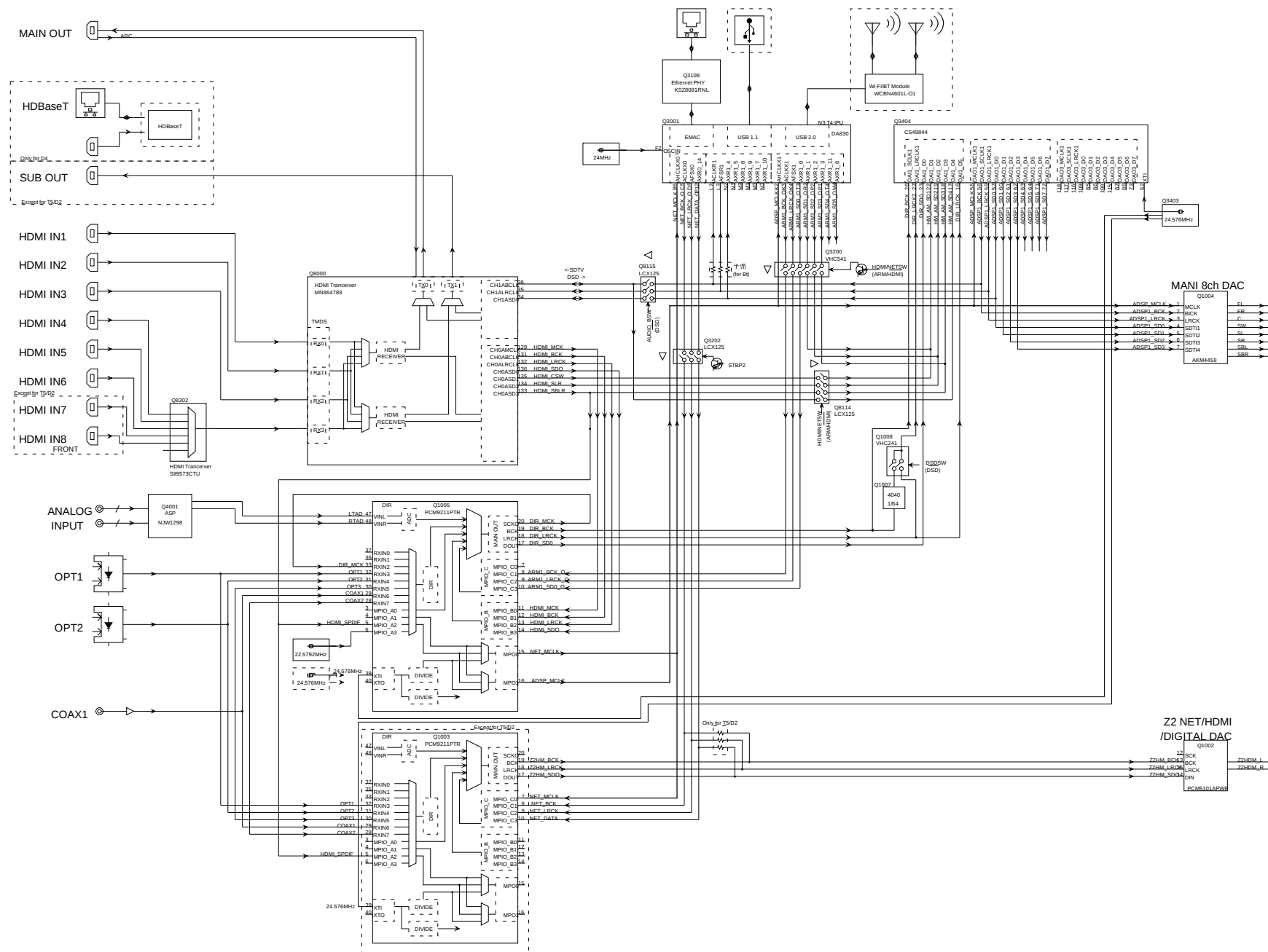
SCHEMATIC DIAGRAM (PART-3) BLOCK DIAGRAM(Digital Aud
