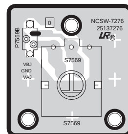
Component side
