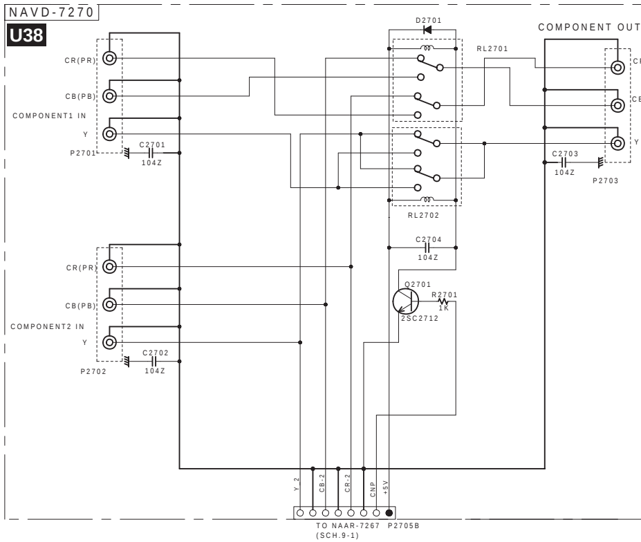
SCHEMATIC DIAGRAM 9-2 Componet video and RS-232C sections
