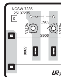
U9 Power switch PC board
