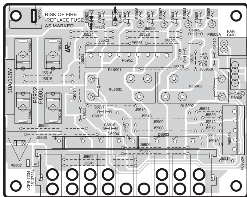
U16 AC inlet terminal PC board
