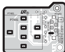
Component side
