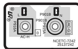
U16 AC inlet terminal PC board
