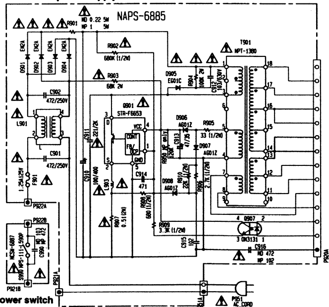
U09 2nd power supply circuit PC board
