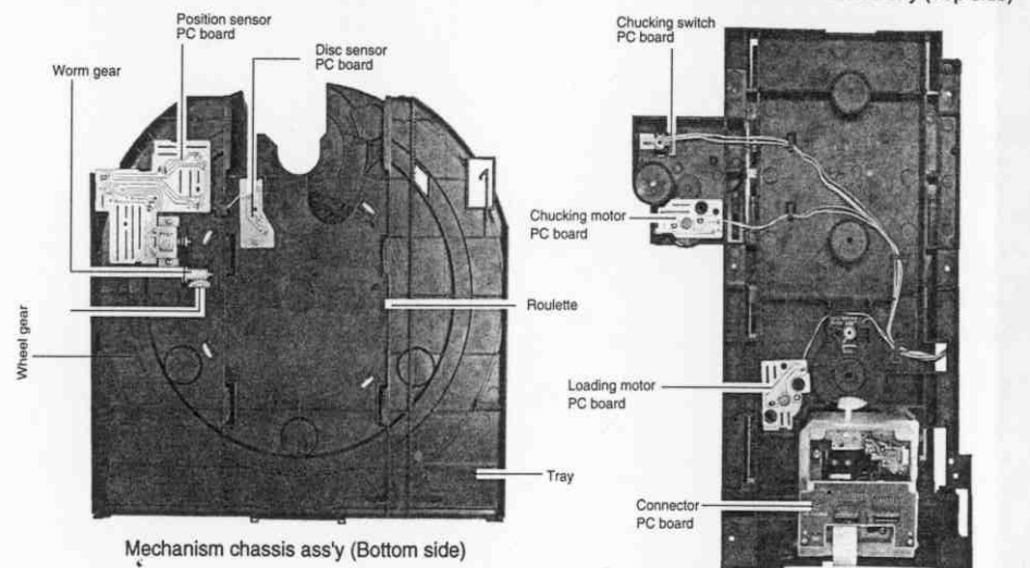
Mechanism chassis ass'y (Bottom side)
