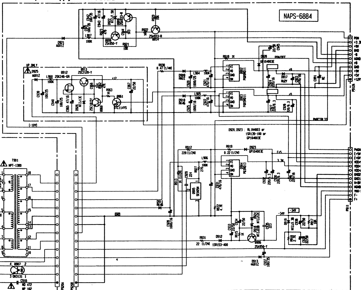
U08 1st power supply circuit PC board
