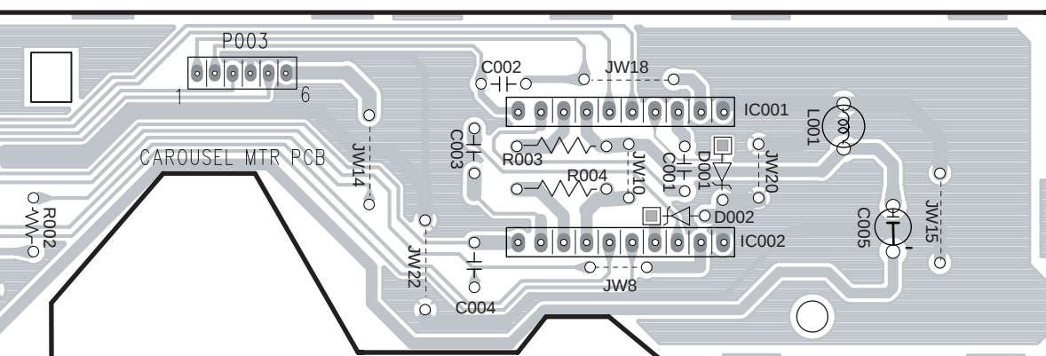
Component side view
