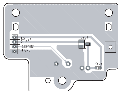
Soldering side
