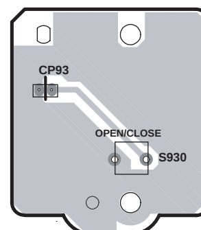
Soldering side
