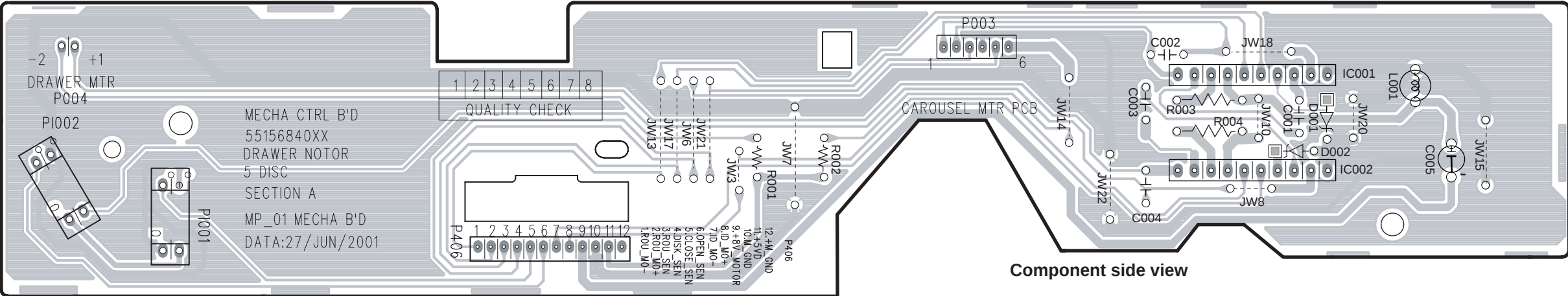
Mechanism control PC board
