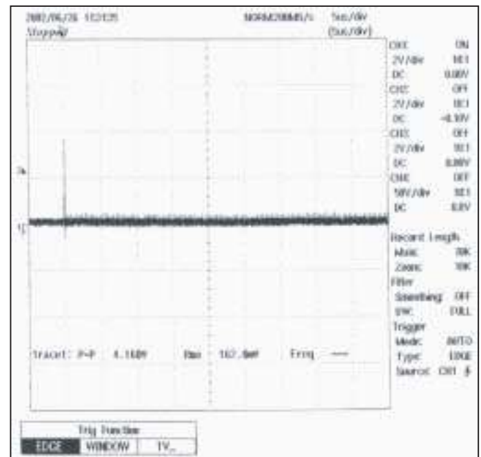
IC21 PIN 19 (SECTOR_START)
