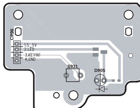
Component side
