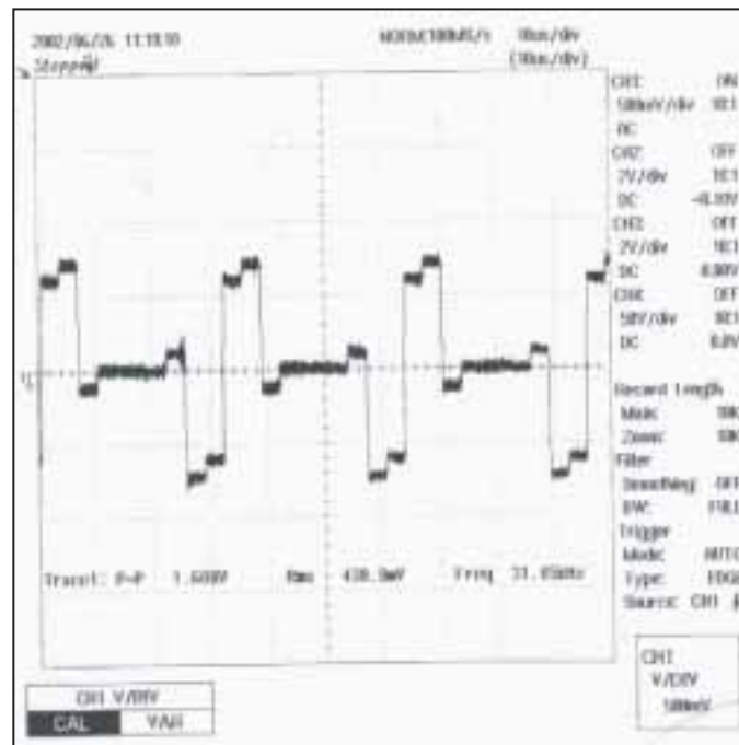
IC12 PIN 19 (Cr)
