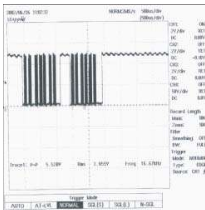
IC22 PIN 6 (IIC_CLK)
