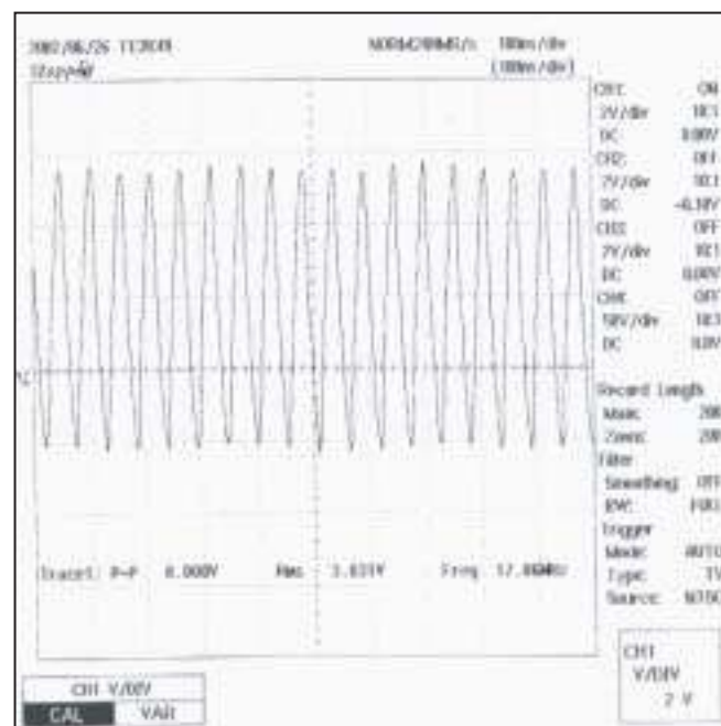
IC21 PIN 55 (PCM_MCLK)
