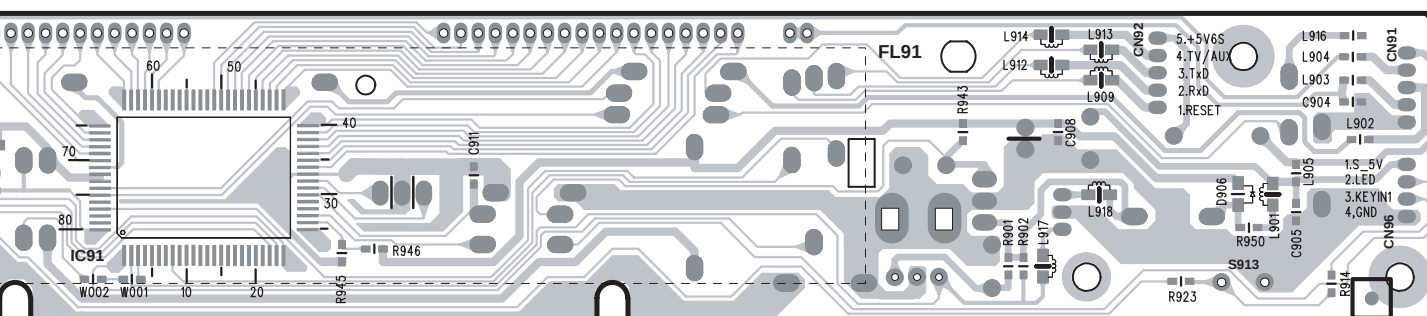
Soldering side
