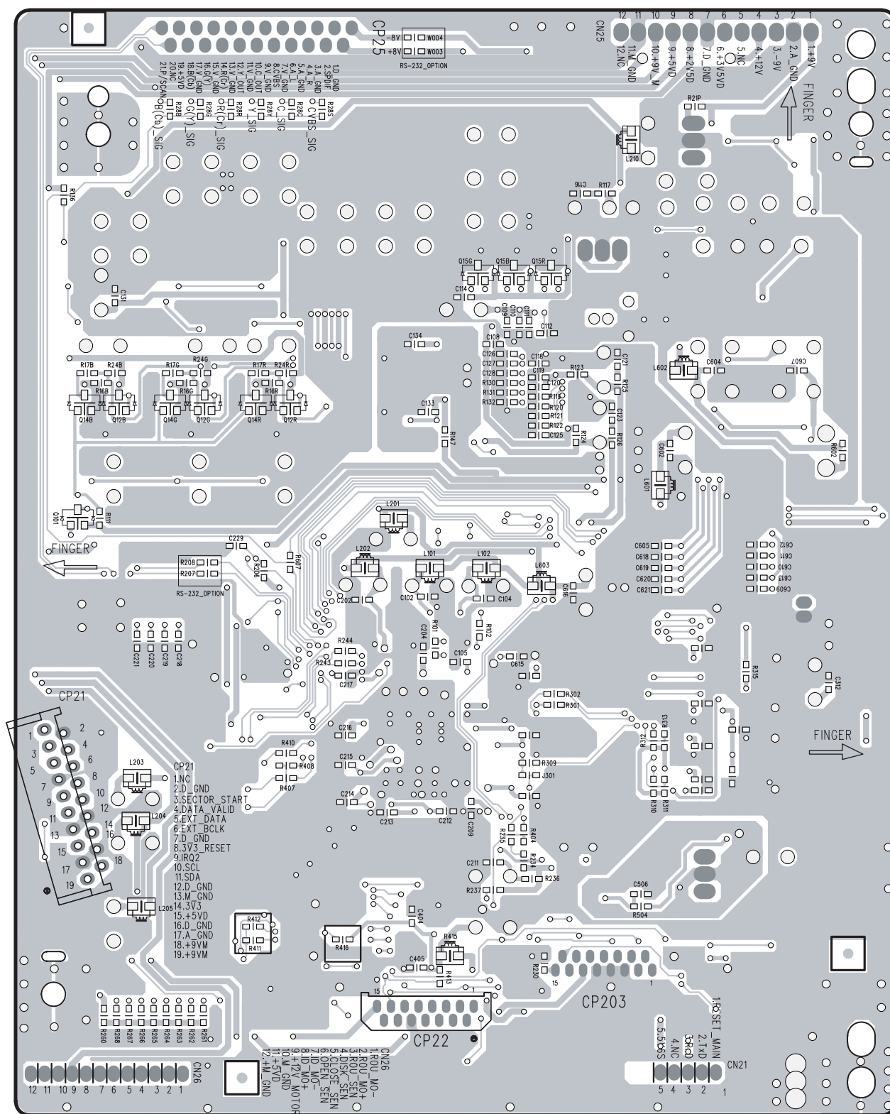
Bottom pattern and Bottom component
