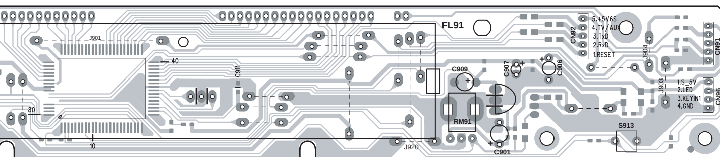
Component side
