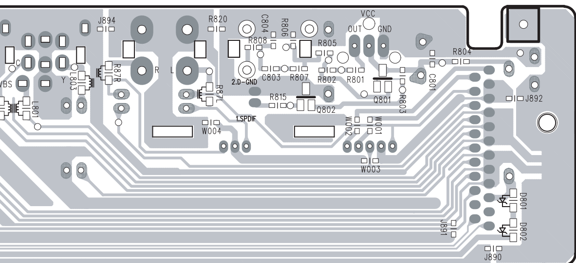
Soldering side
