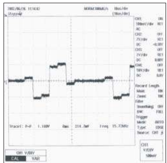
IC12 PIN 19 (Cr)
