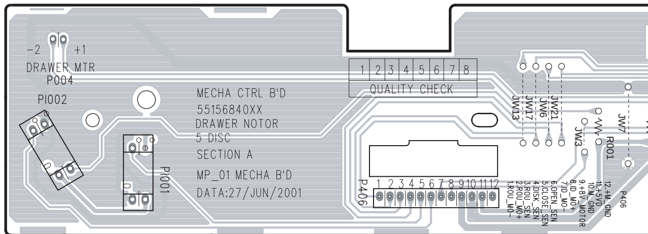
Mechanism control PC board
