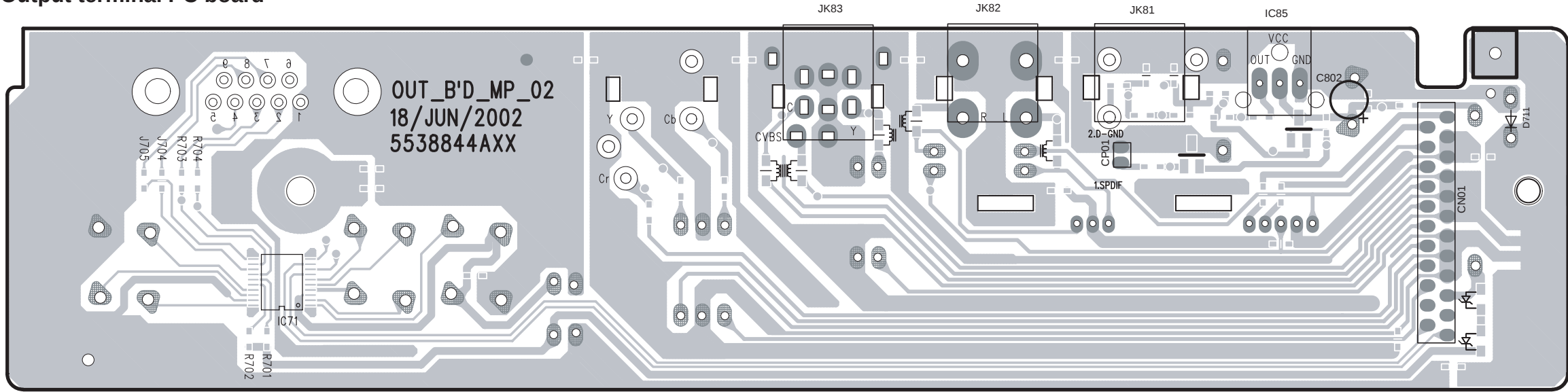
Component side
