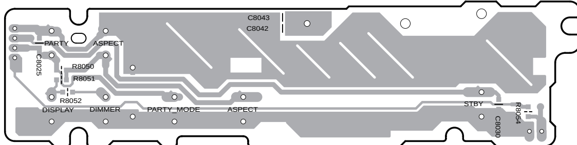
Soldering side view
