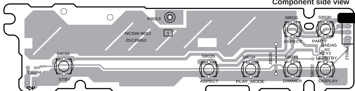
Component side view
