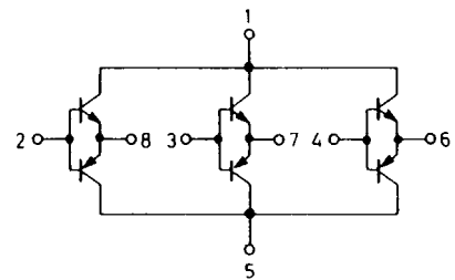
STA341M-L (Transistor array)
