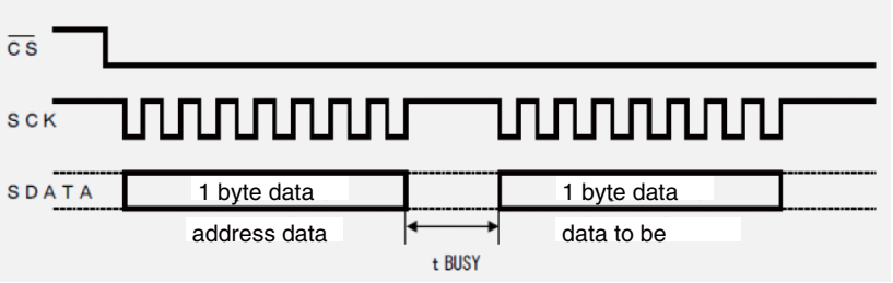
Timing of Serial Communication
