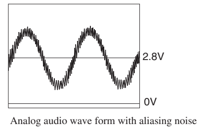
WF09 DAC_OUT-
