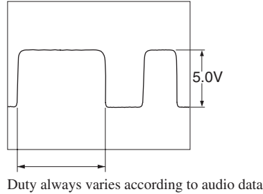
WF05 SAI_SLCK
