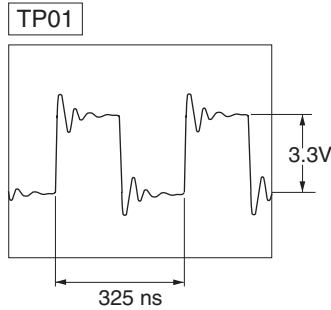
WF05 SAI_SLCK
