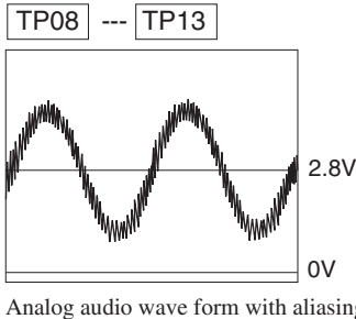
WF10 AUDIO_FL
