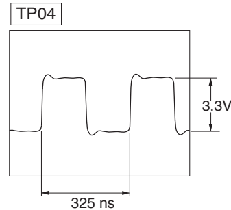
WF08 CX_SCLCK
