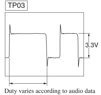
WF03 SAI_SDOUT
