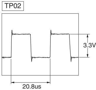
WF04 SAI_LRCK
