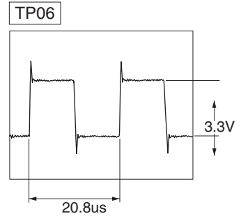
WF06 CX_SDIN1
