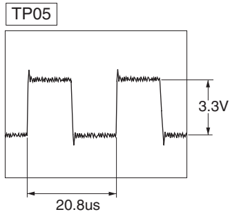
WF07 CX_LRCK
