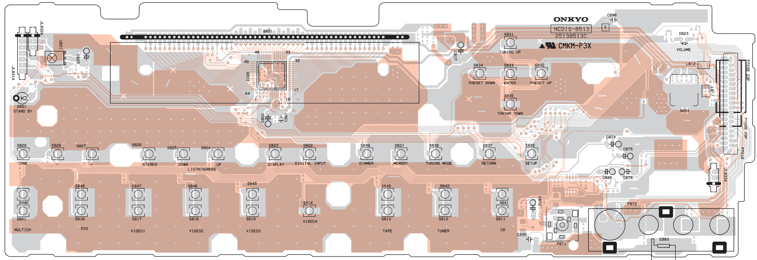
U01 DISPLAY PC BOARD (NADIS-8513) Side A
