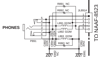
U04 HEADPHONE JACK PC BOARD
