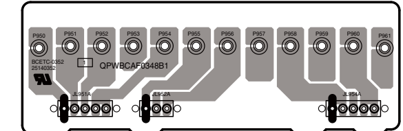
U0014 BAETC-0352 (TRANS TRM PC BOARD) A-side(Component side)
