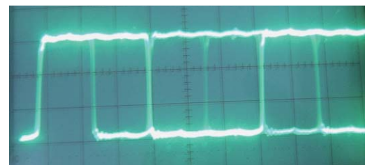
HDMI_SPDIF
