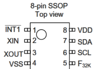
Figure 2 Pin assignment
