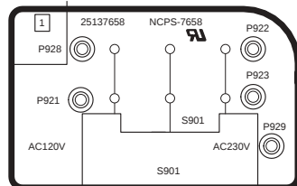
U007:PS-7658 Component side
