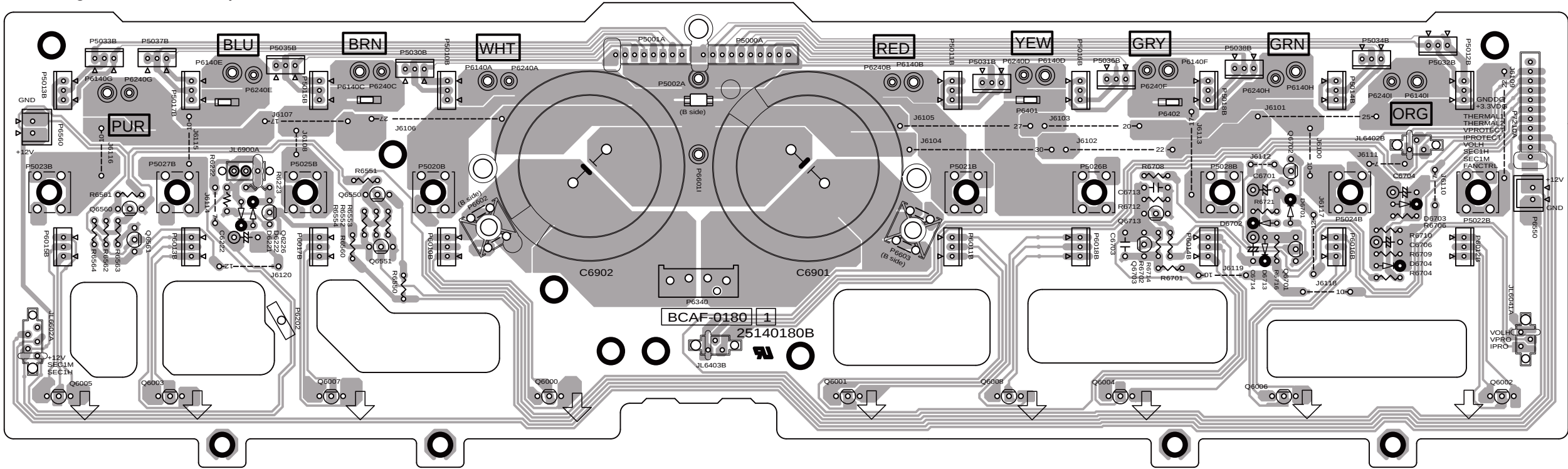
U0010 AMP-4 POWER SUPPLY PC BOARD (BAAF-0180-1C)
