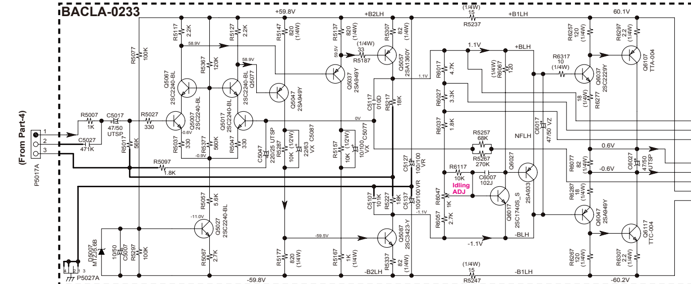
U0037 VOLTAGE AMP PC BOARD BACLA-0233
