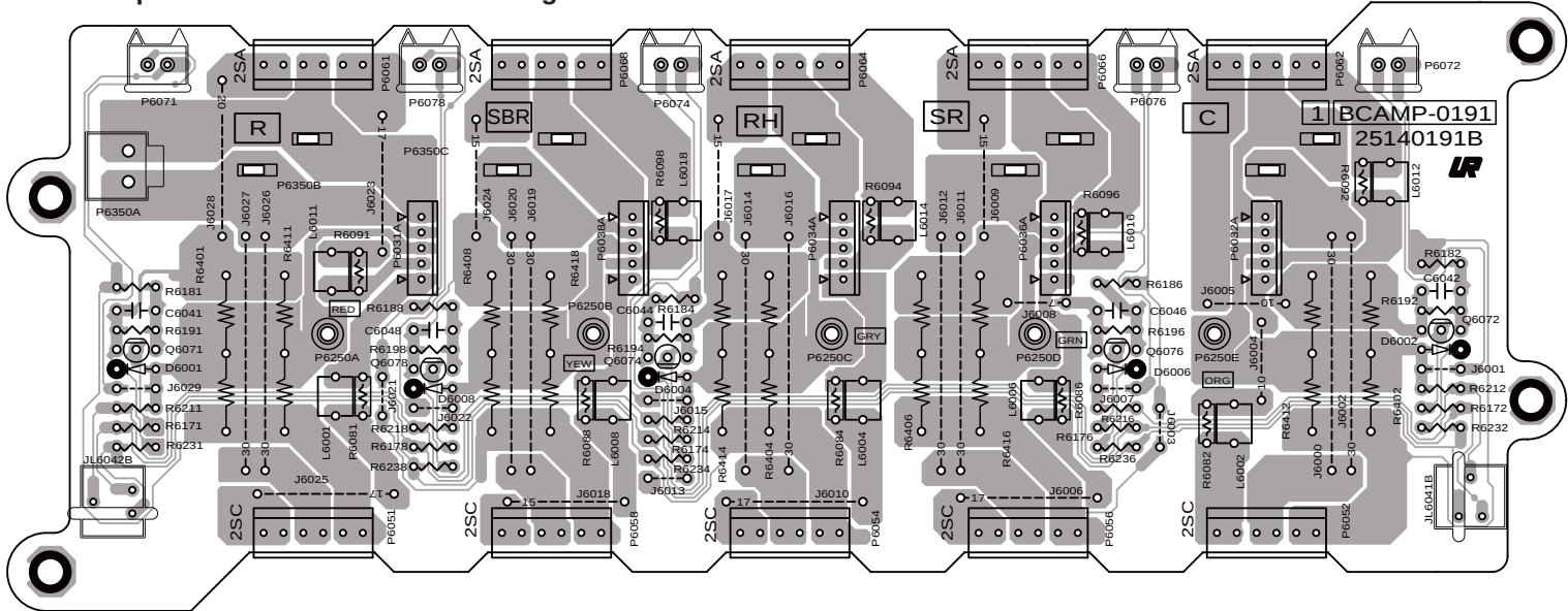
Component side view from soldering side
