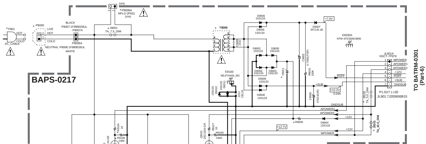
TX-NR5007/NA5007,DTR-80.1 Transformer
