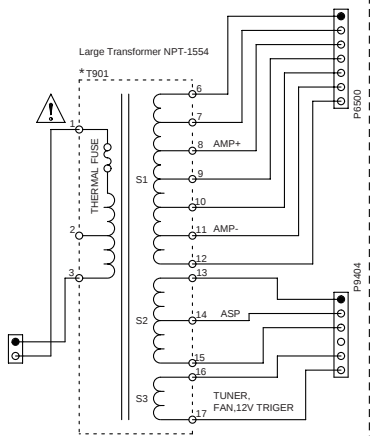
TX-NR5007/NA5007,DTR-80.1 Transformer
