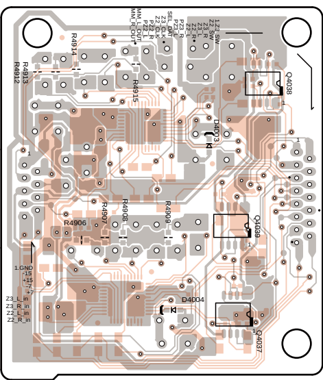
Soldering side view from component side
