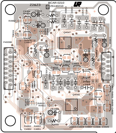
Component side view from soldering side
