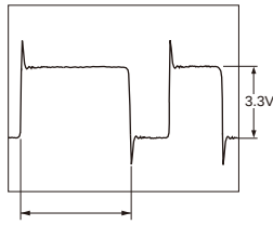
(WF03) SAI_SDOUT/DIR_SDOUT (SD-12:G8)
