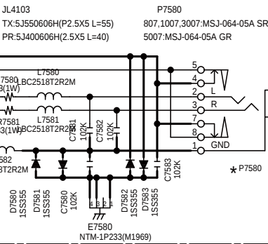
U0052 PHONE JACK PC BOARD
