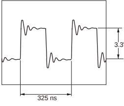
(WF05) SAI_SLCK/DIR_BCK (SD-12:F8)
