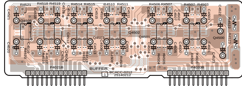
Component side view from soldering side
