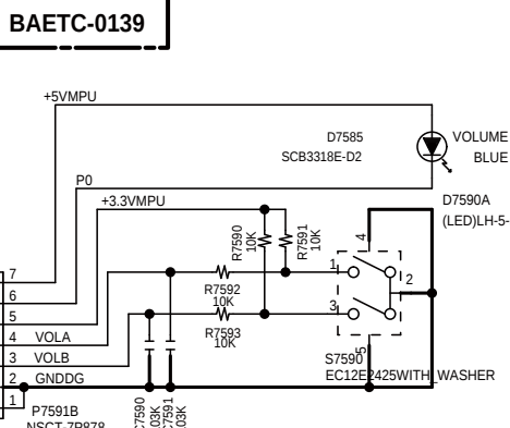
U0054 VOLUME PC BOARD
