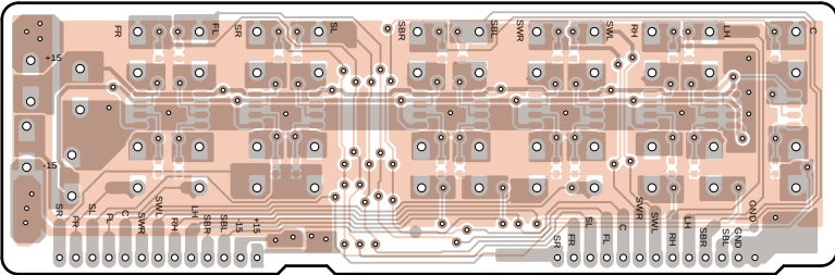
Soldering side view from component side
