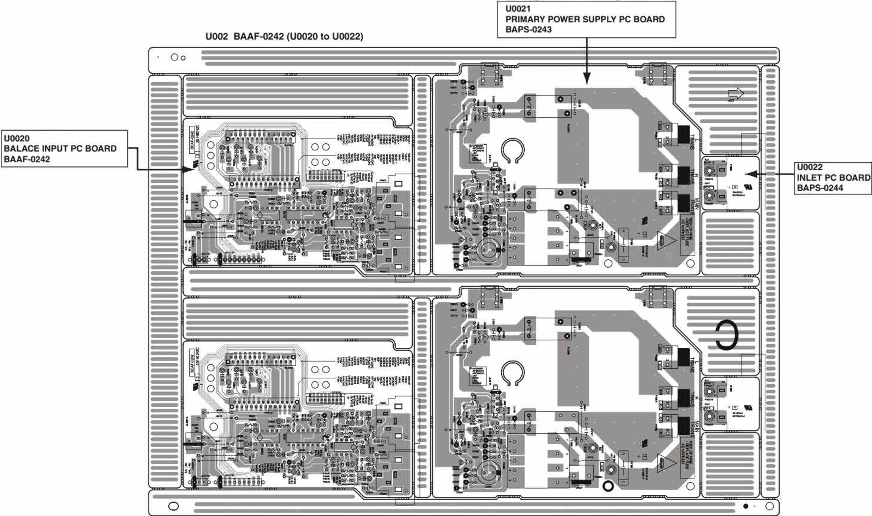
Component side view from soldering side
