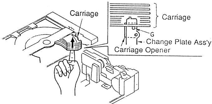
Fig. 2.7.4 Leveling the carriages at the right side
