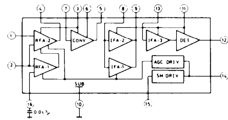
\mu PC1243C (AM radio system)
