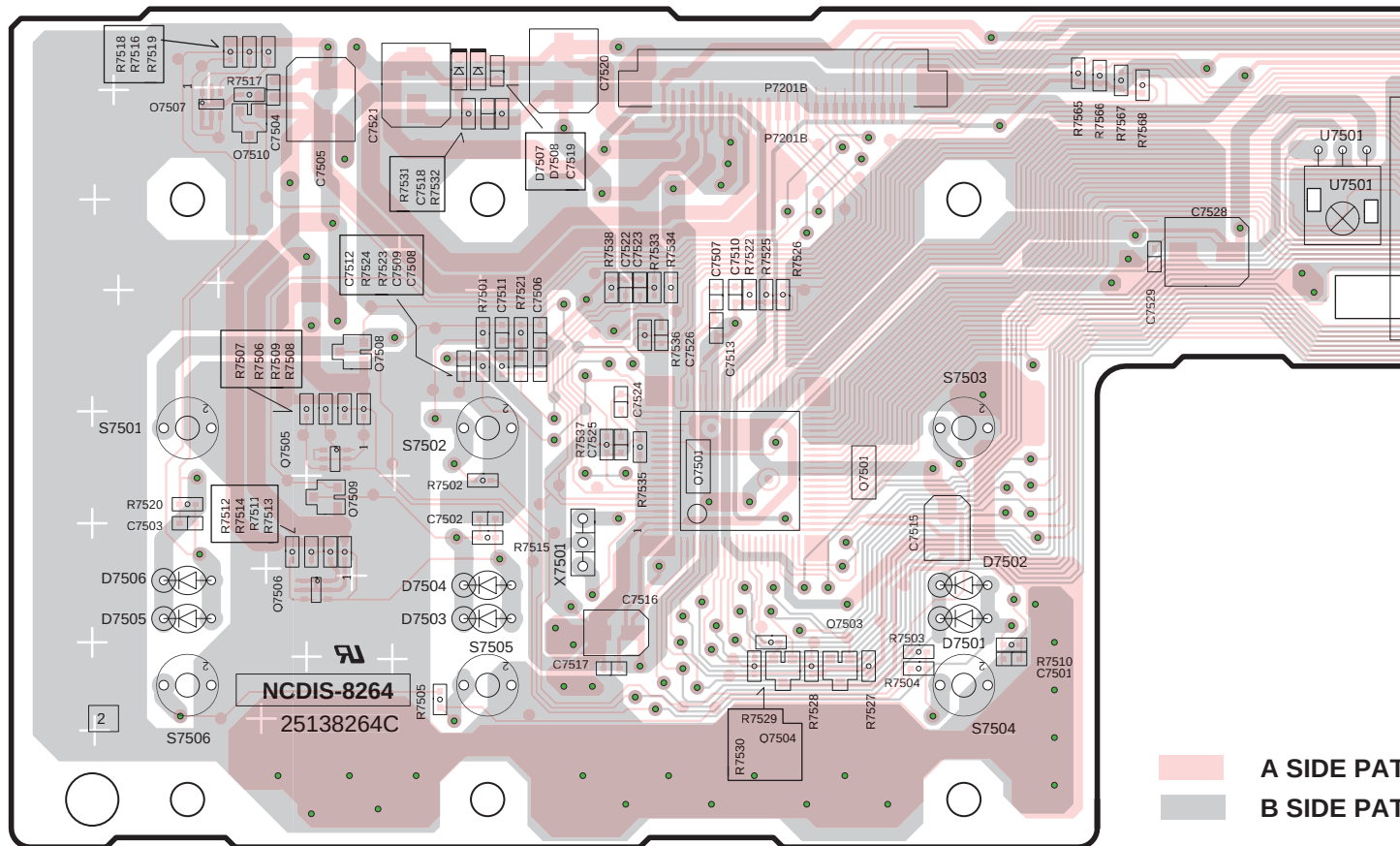
B-SIDE PATTERN AND A-SIDE SILK SCREEN
