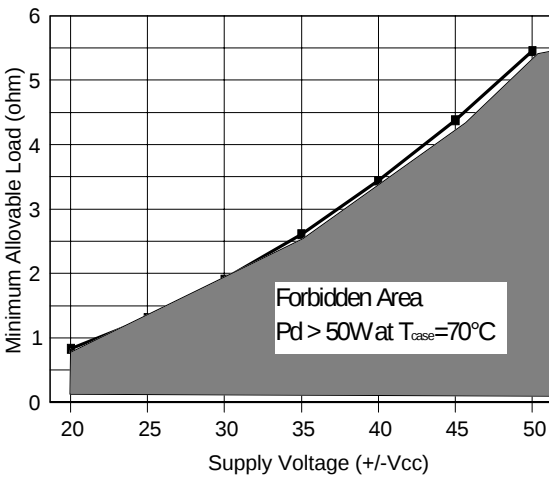
Figure 13: Modular Application Pd vs Vsupply (ref. fig. 7)
