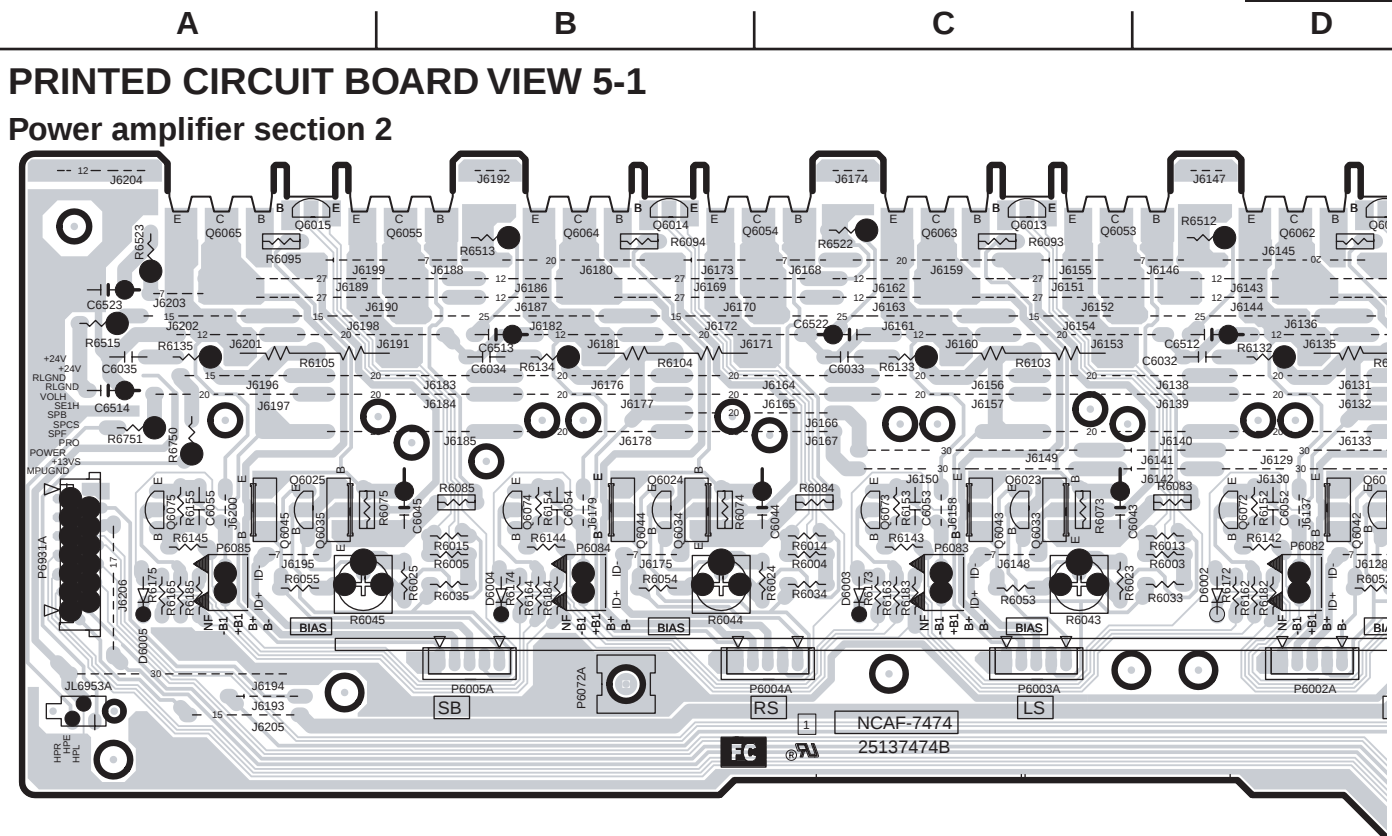
U15 Power amplifier PC board
